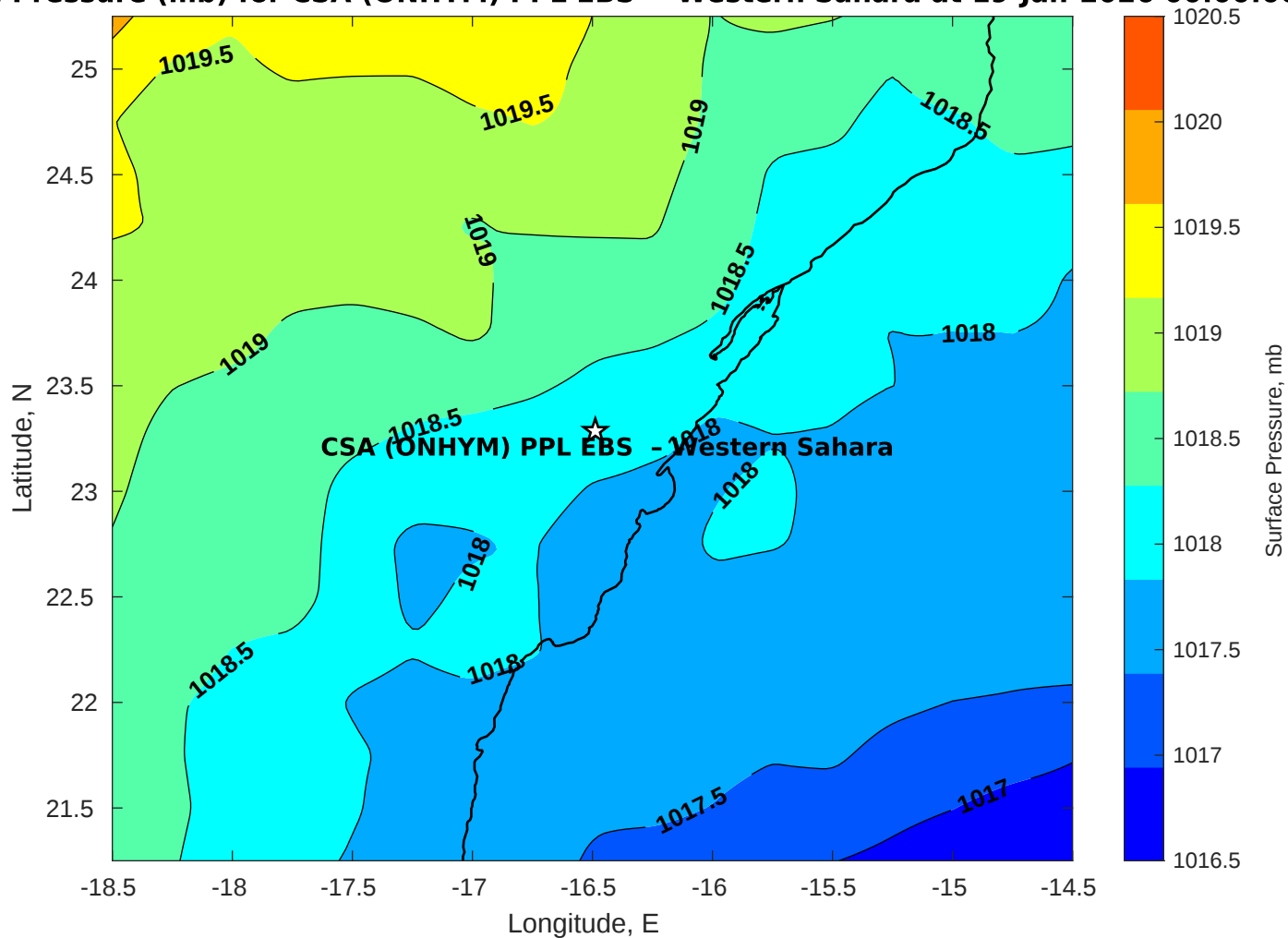
Surface Pressure (mb) for CSA (ONHYM) PPL EBS - Western Sahara at 19-Jan-2026 00:00:00
