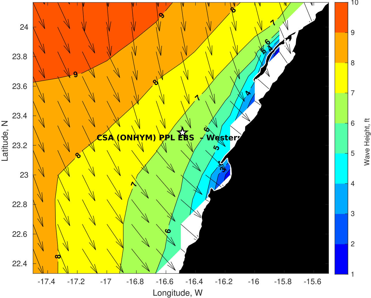
GFS Wave Height (ft) for CSA (ONHYM) PPL EBS - Western Sahara at 19-Jan-2026 09:00:00
