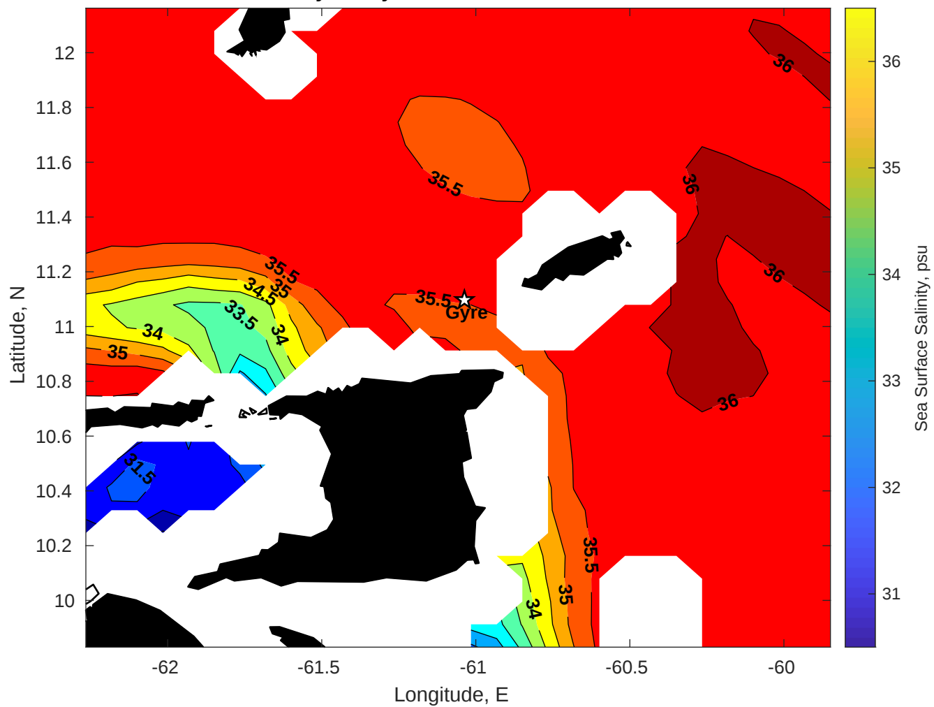
Surface Salinity for Gyre at 18-Jan-2026 00:00:00
