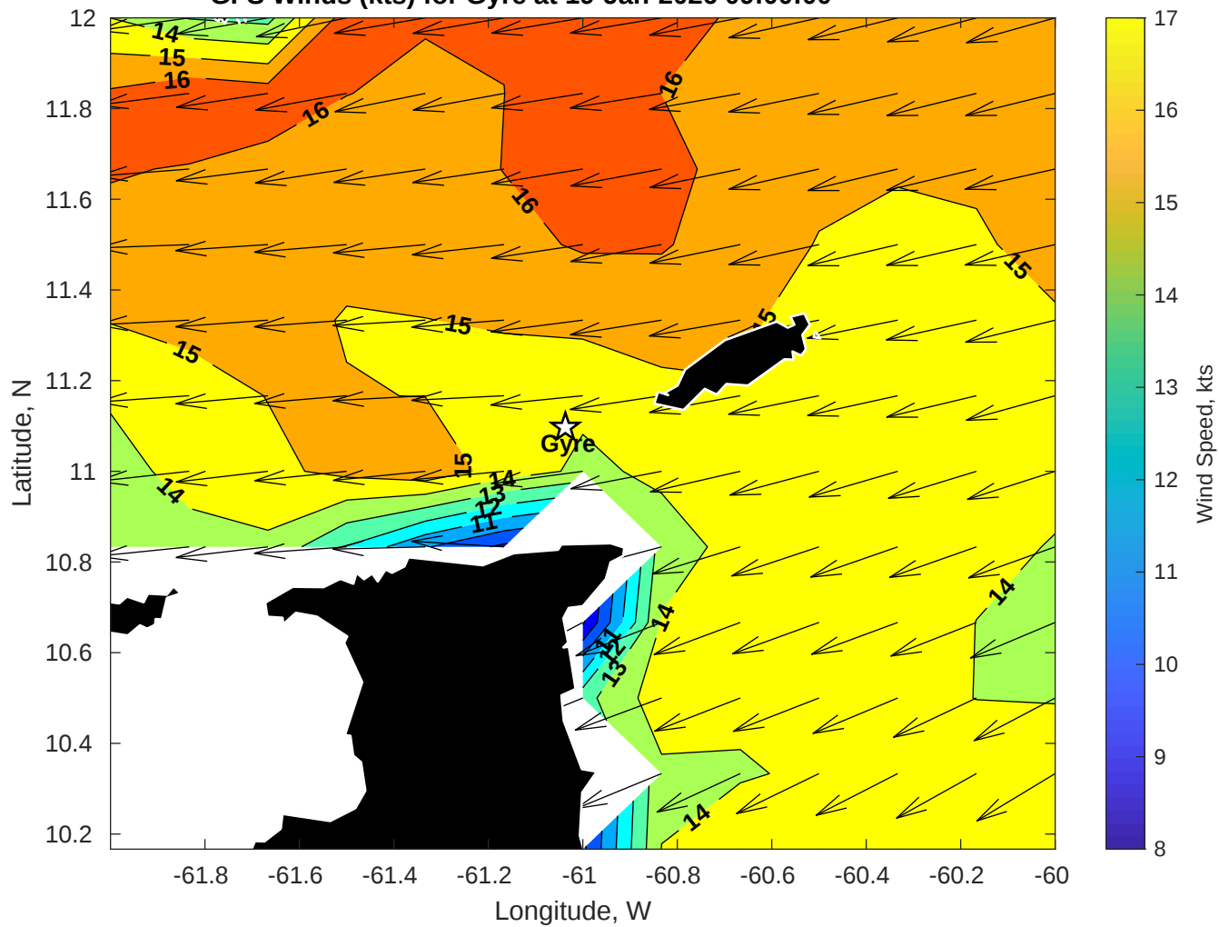
GFS Winds (kts) for Gyre at 19-Jan-2026 09:00:00
