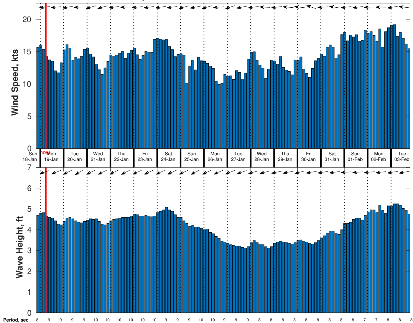
Wind & Wave Forecast for Gyre from 18-Jan-2026 20:00:00 to 03-Feb-2026 20:00:00
