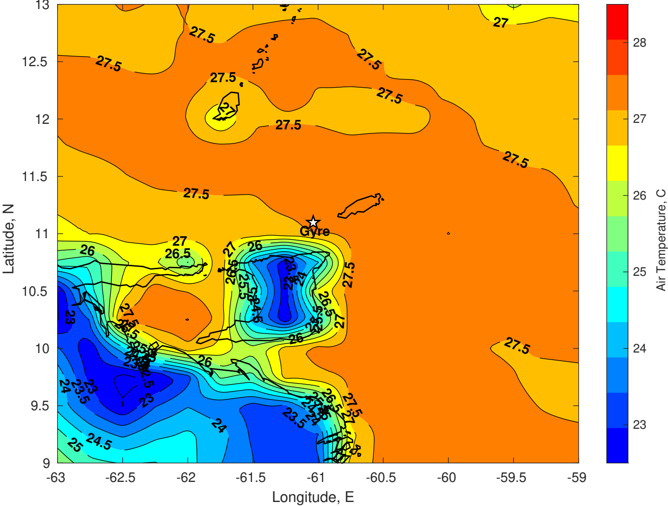
Air Temperature (C) for Gyre at 19-Jan-2026
