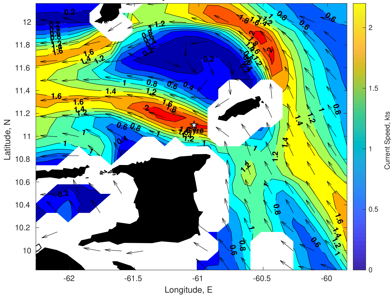
Surface Currents for Gyre at 18-Jan-2026 00:00:00
