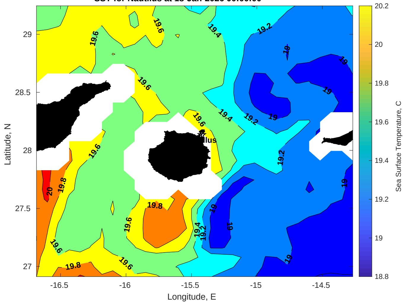
SST for Nautilus at 18-Jan-2026 00:00:00
