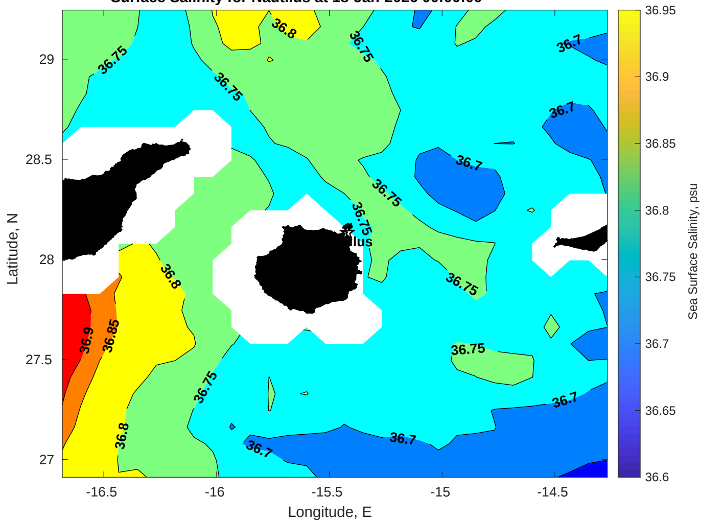
Surface Salinity for Nautilus at 18-Jan-2026 00:00:00
