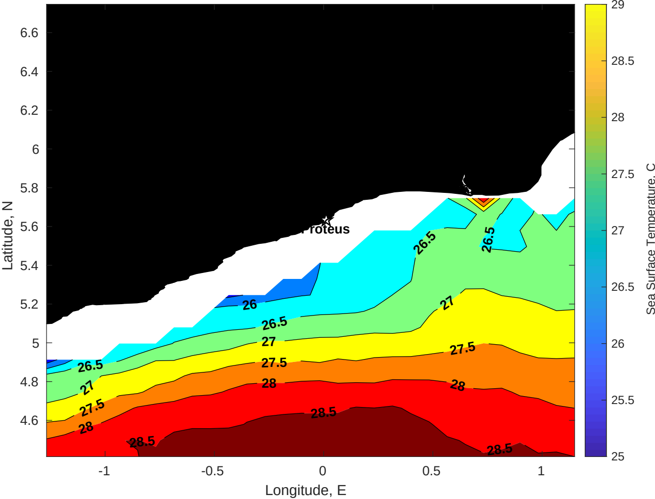
SST for Proteus at 18-Jan-2026 00:00:00
