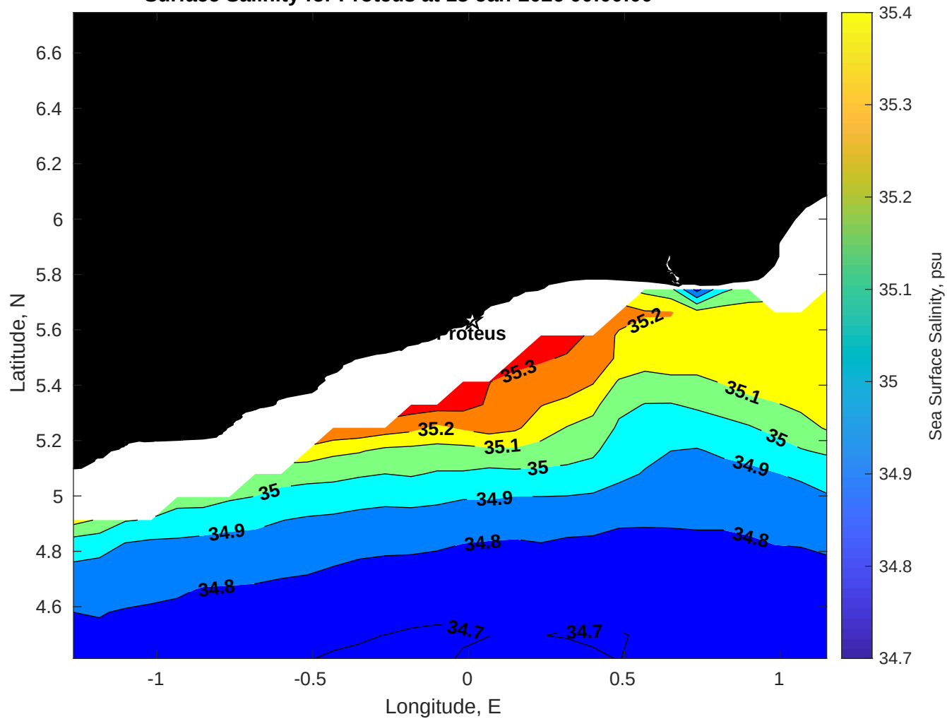
Surface Salinity for Proteus at 18-Jan-2026 00:00:00
