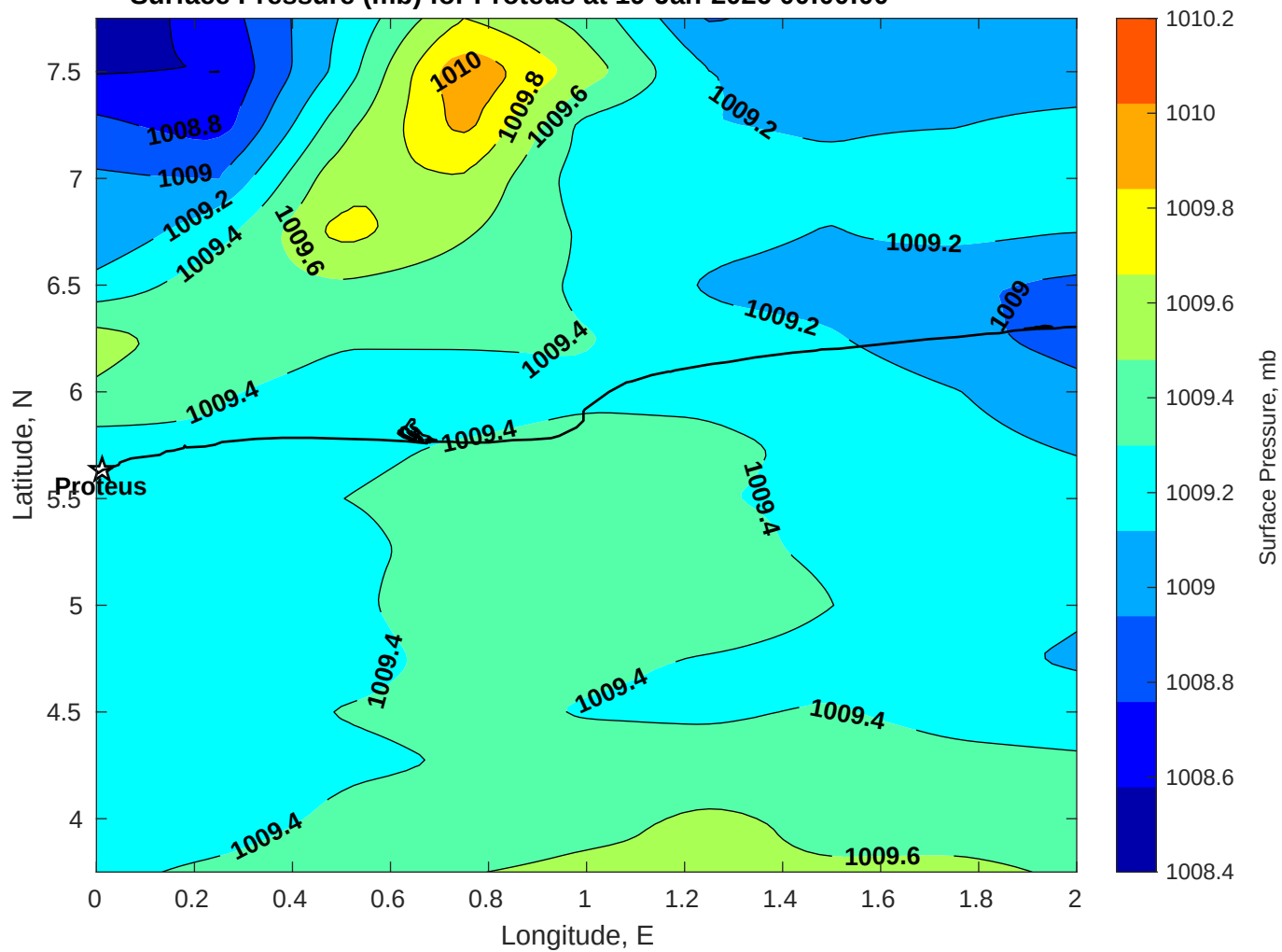
Surface Pressure (mb) for Proteus at 19-Jan-2026 00:00:00
