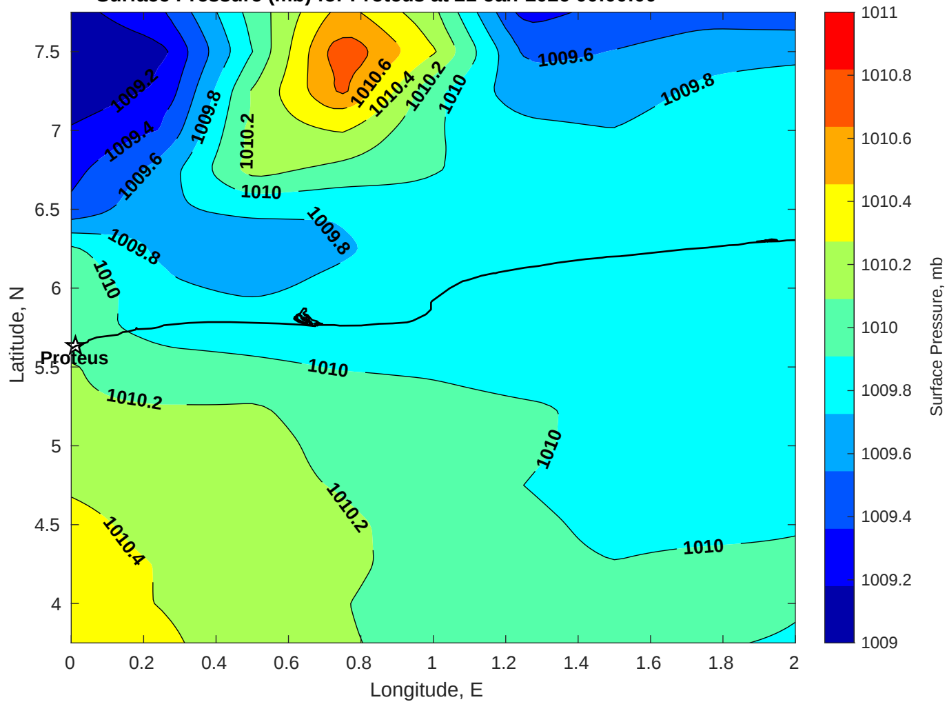
Surface Pressure (mb) for Proteus at 21-Jan-2026 00:00:00
