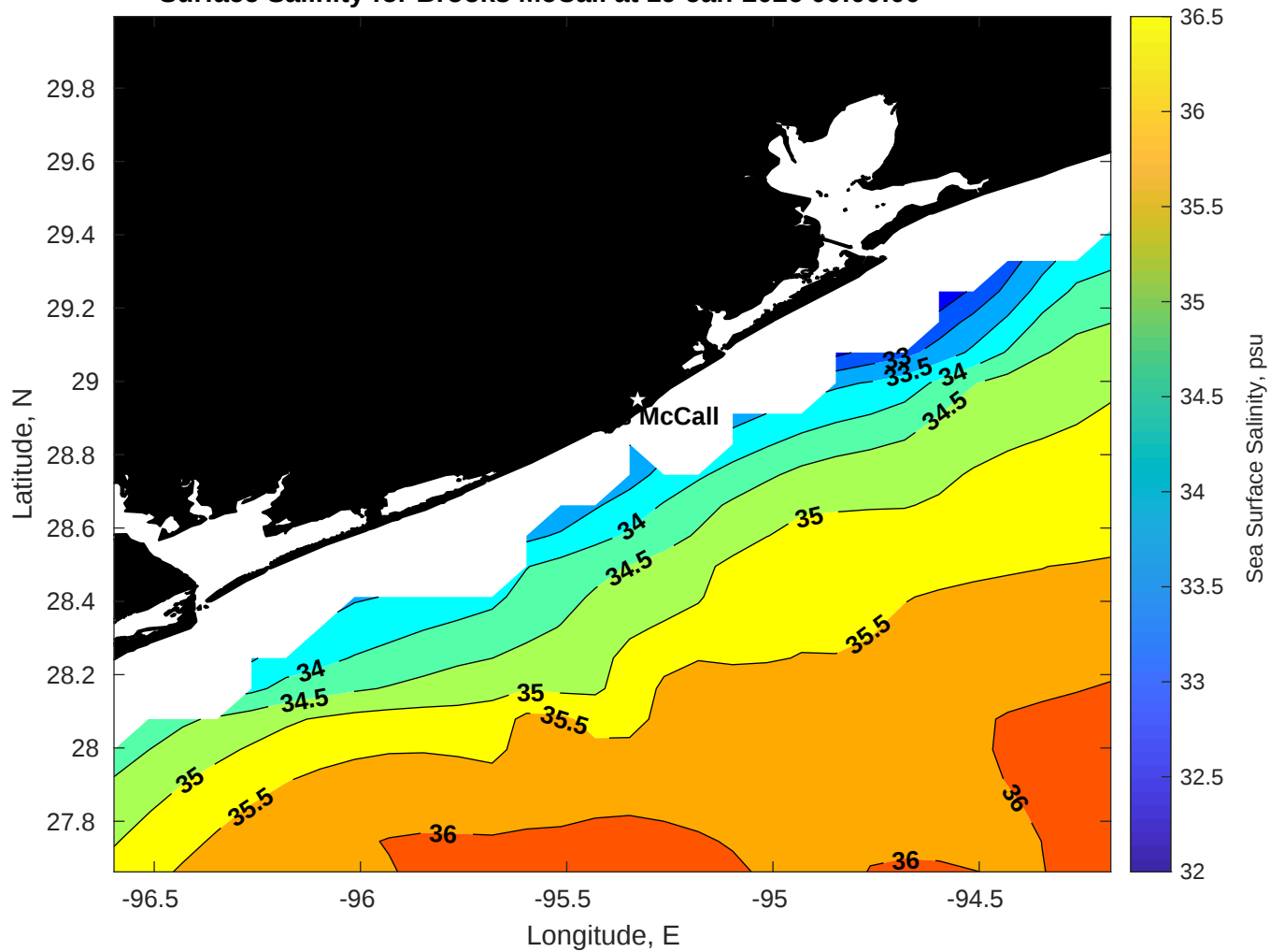
Surface Salinity for Brooks McCall at 19-Jan-2026 00:00:00
