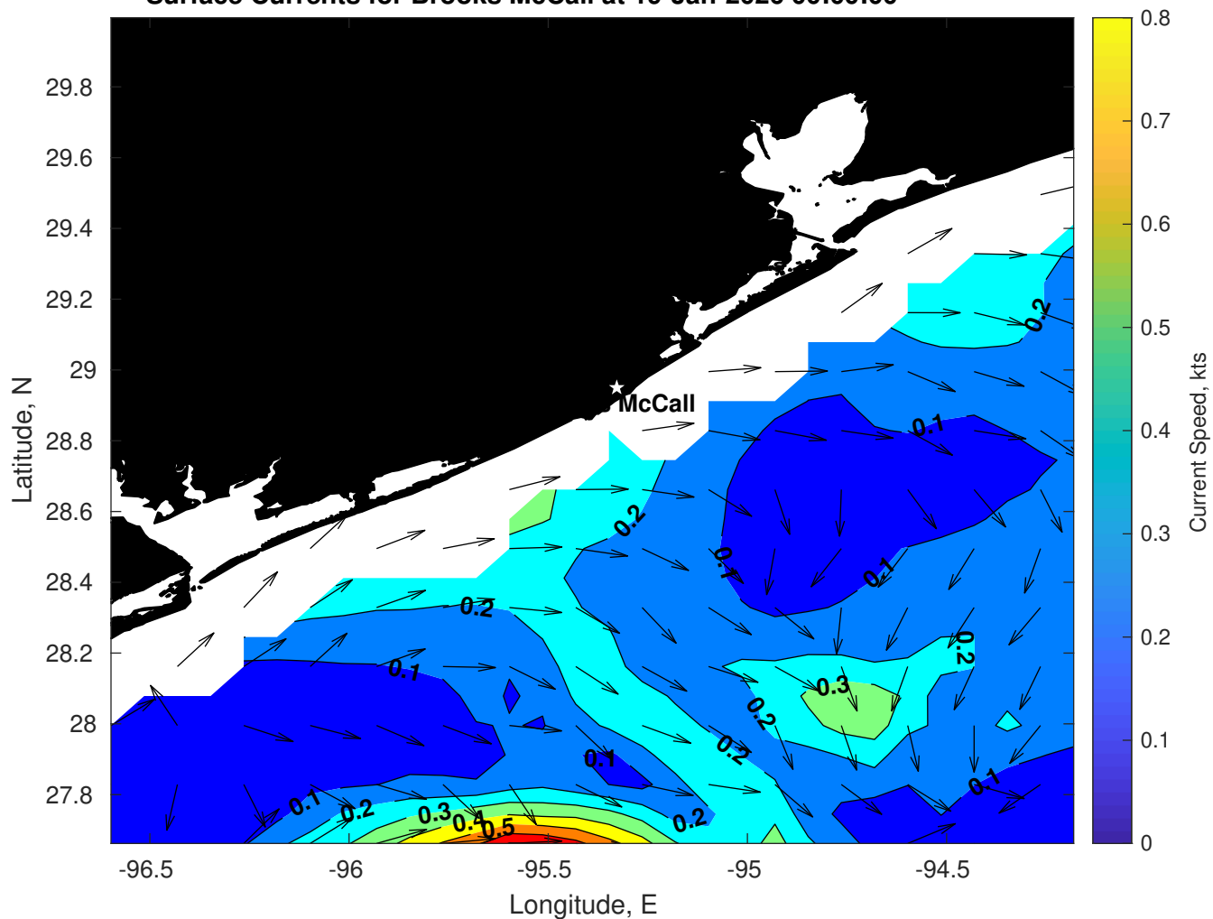
Surface Currents for Brooks McCall at 19-Jan-2026 00:00:00
