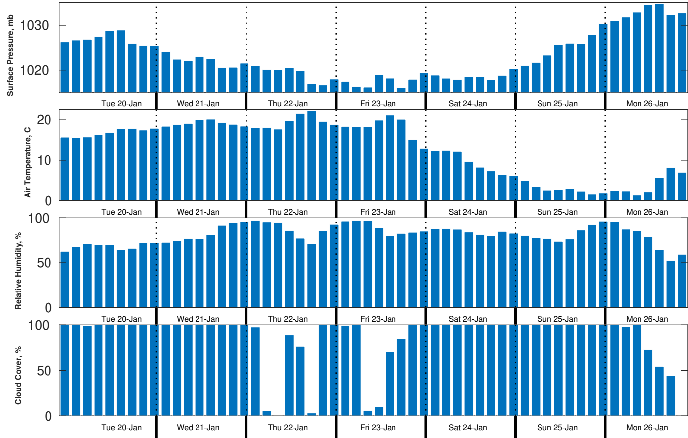
Met Forecast for Brooks McCall from 20-Jan-2026 00:00:00 to 27-Jan-2026 00:00:00
