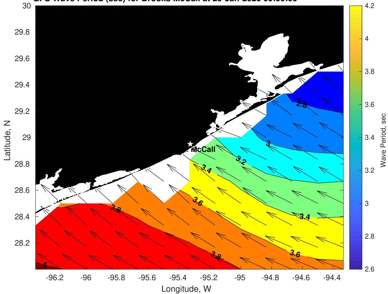
GFS Wave Period (sec) for Brooks McCall at 20-Jan-2026 09:00:00
