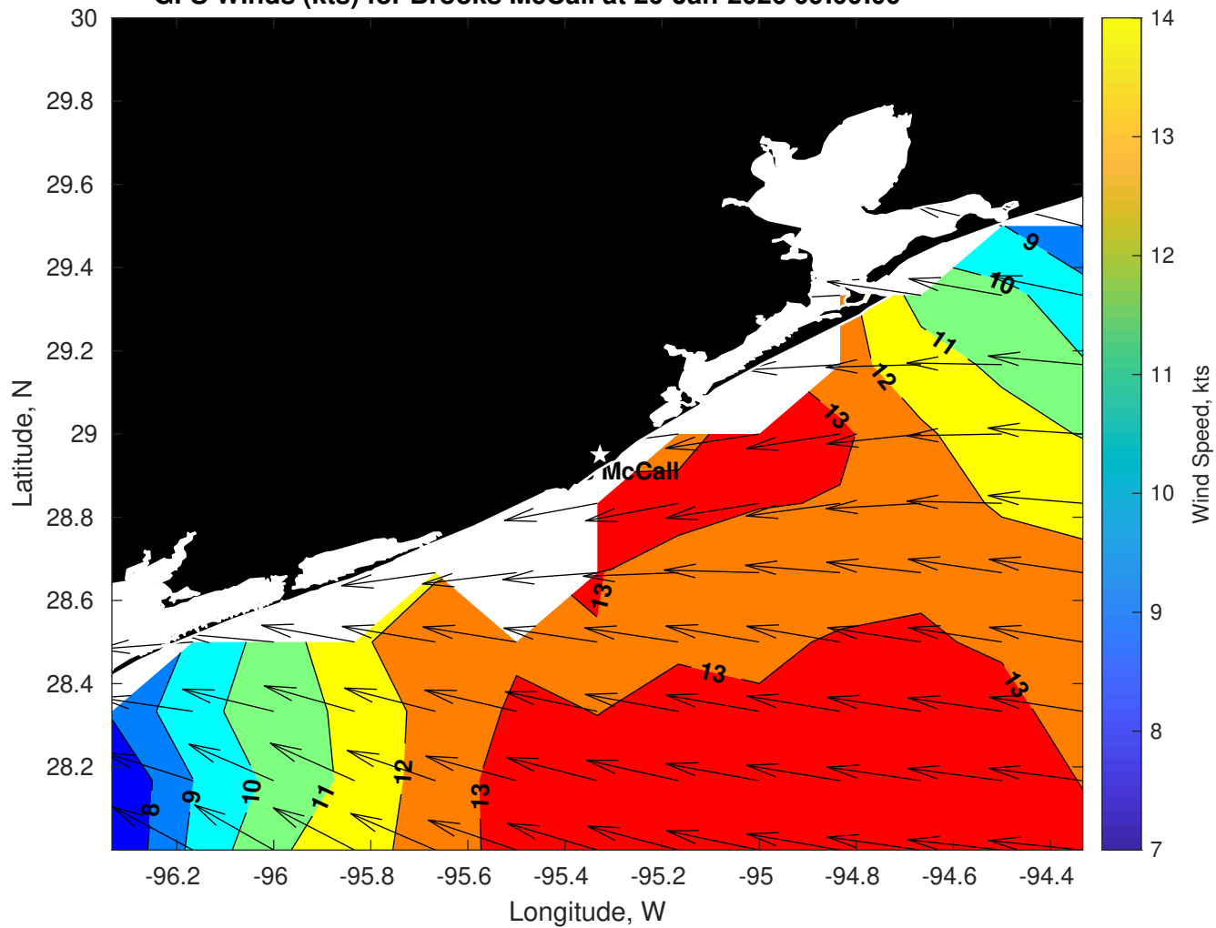
GFS Winds (kts) for Brooks McCall at 20-Jan-2026 09:00:00
