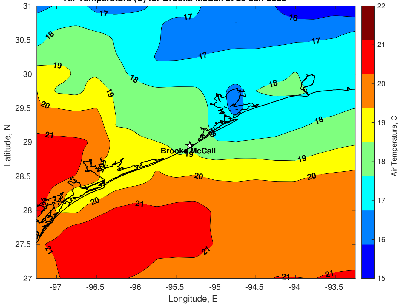
Air Temperature (C) for Brooks McCall at 20-Jan-2026
