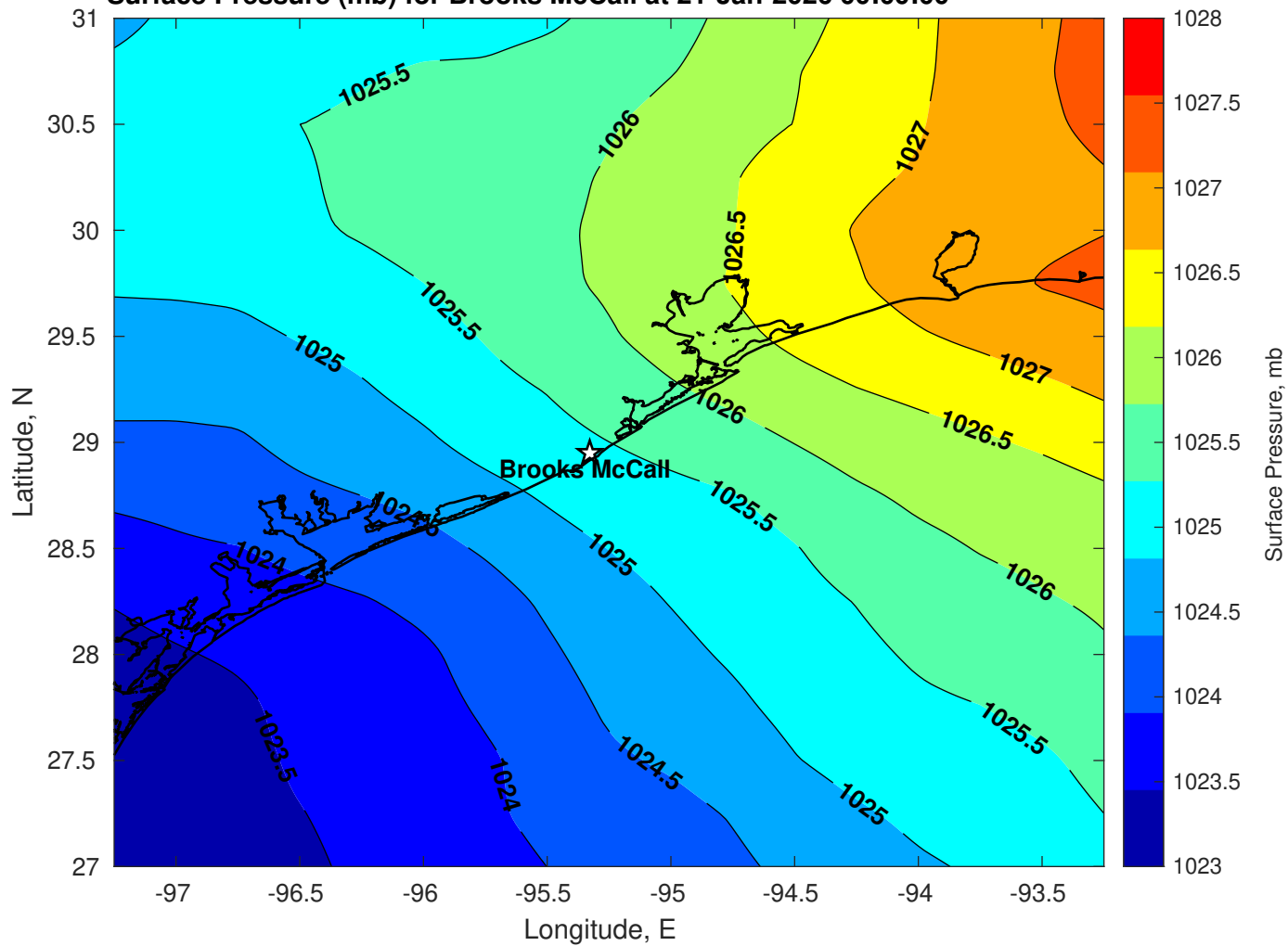
Surface Pressure (mb) for Brooks McCall at 21-Jan-2026 00:00:00
