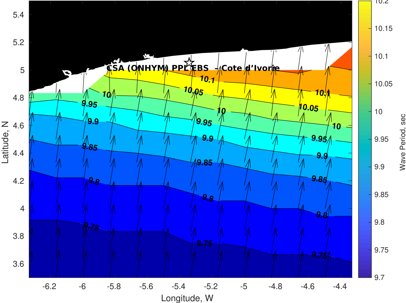
GFS Wave Period (sec) for CSA (ONHYM) PPL EBS - Cote d'Ivoire at 20-Jan-2026 09:00:00
