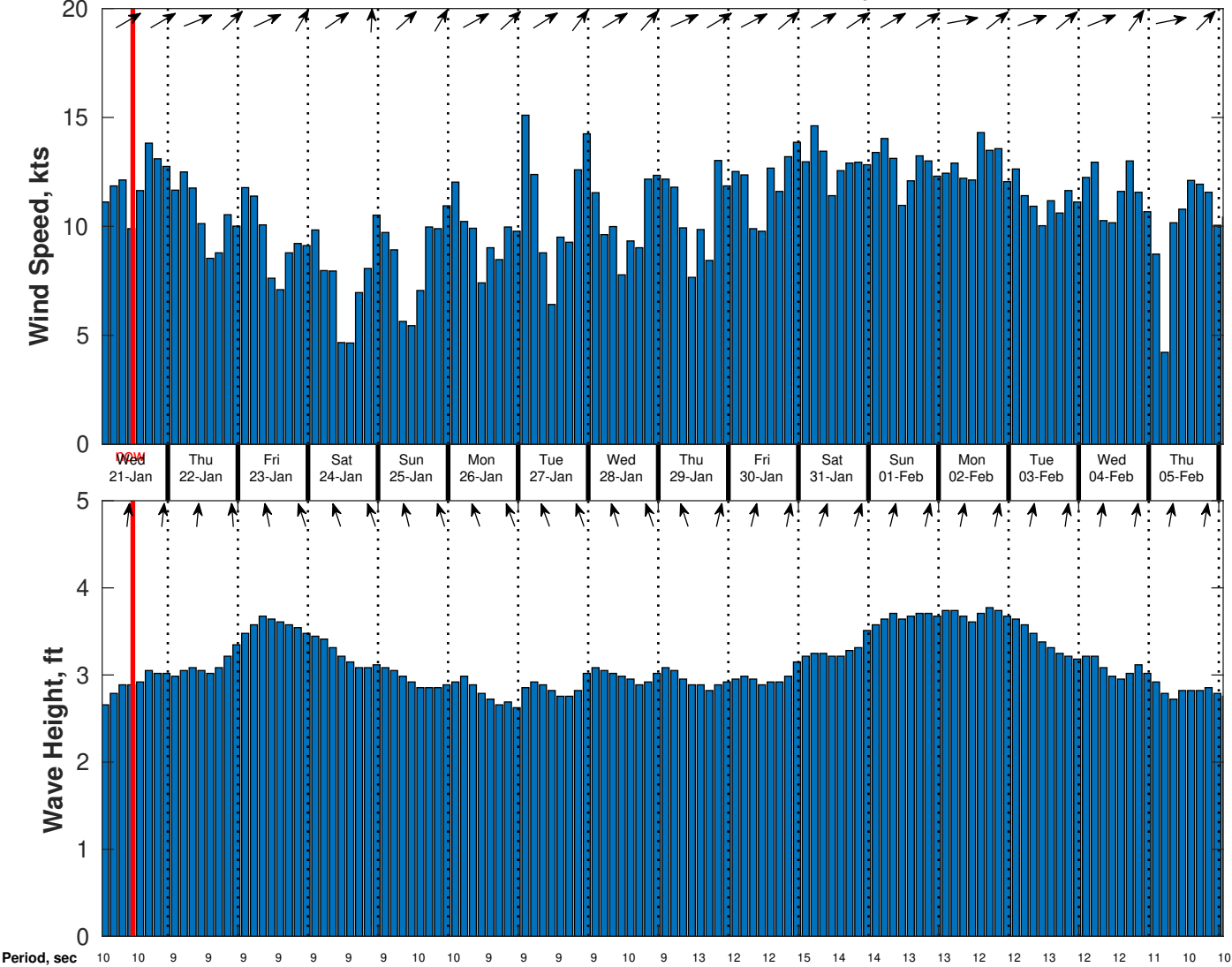
Wind & Wave Forecast for CSA (ONHYM) PPL EBS - Cote d'Ivoire from 20-Jan-2026 01:00:00 to 05-Feb-2026 01:00:00
