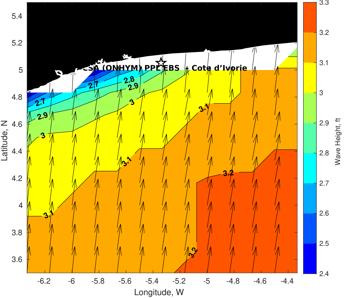
GFS Wave Height (ft) for CSA (ONHYM) PPL EBS - Cote d'Ivoire at 20-Jan-2026 09:00:00
