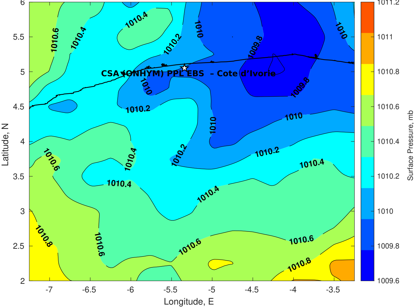
Surface Pressure (mb) for CSA (ONHYM) PPL EBS - Cote d'Ivoire at 22-Jan-2026 00:00:00
