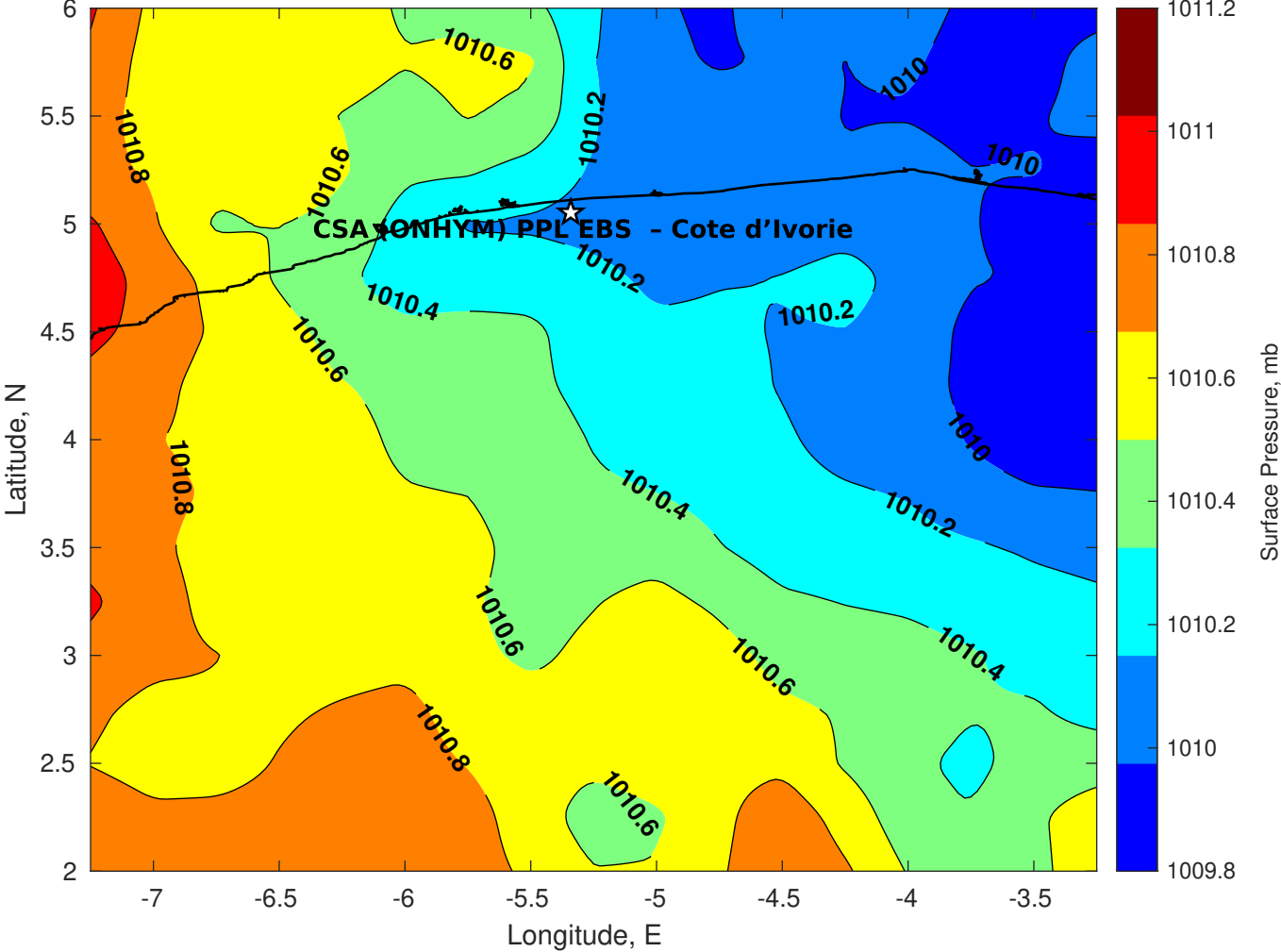
Surface Pressure (mb) for CSA (ONHYM) PPL EBS - Cote d'Ivoire at 20-Jan-2026 00:00:00
