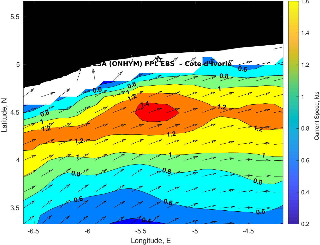
Surface Currents for CSA (ONHYM) PPL EBS - Cote d'Ivoire at 19-Jan-2026 00:00:00
