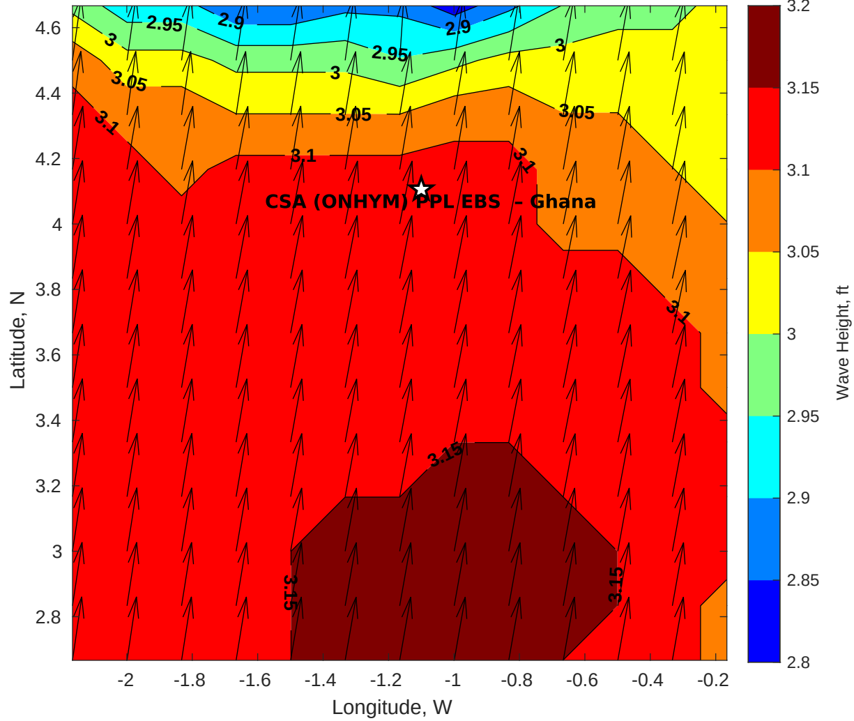
GFS Wave Height (ft) for CSA (ONHYM) PPL EBS - Ghana at 20-Jan-2026 09:00:00
