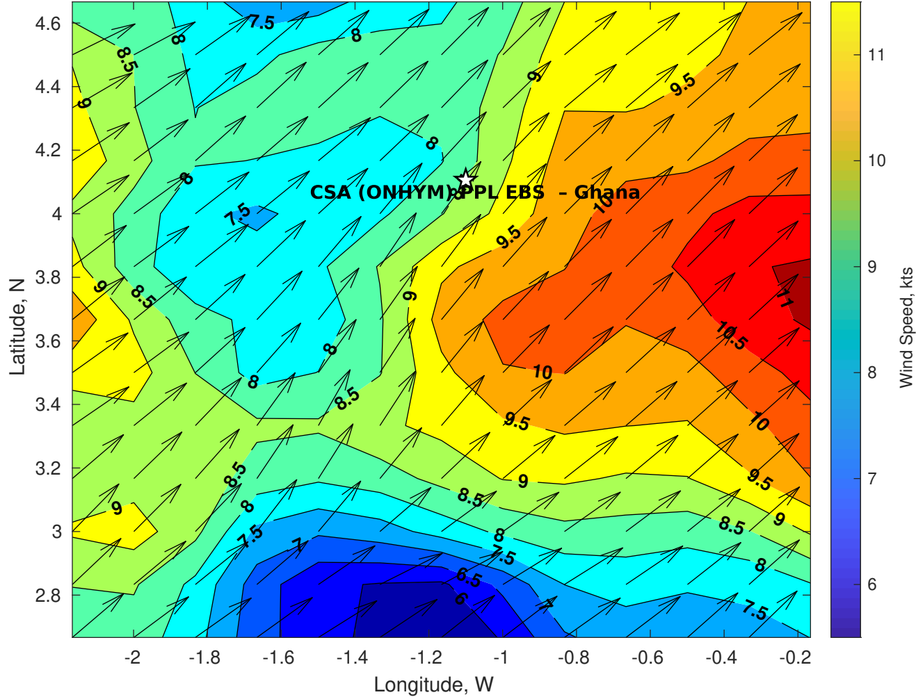
GFS Winds (kts) for CSA (ONHYM) PPL EBS - Ghana at 20-Jan-2026 09:00:00
