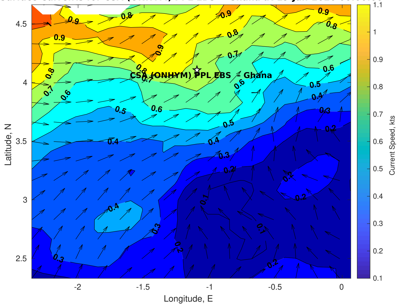
Surface Currents for CSA (ONHYM) PPL EBS - Ghana at 19-Jan-2026 00:00:00
