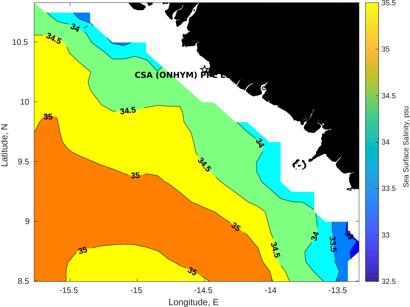
Surface Salinity for CSA (ONHYM) PPL EBS - Guinea at 19-Jan-2026 00:00:00
