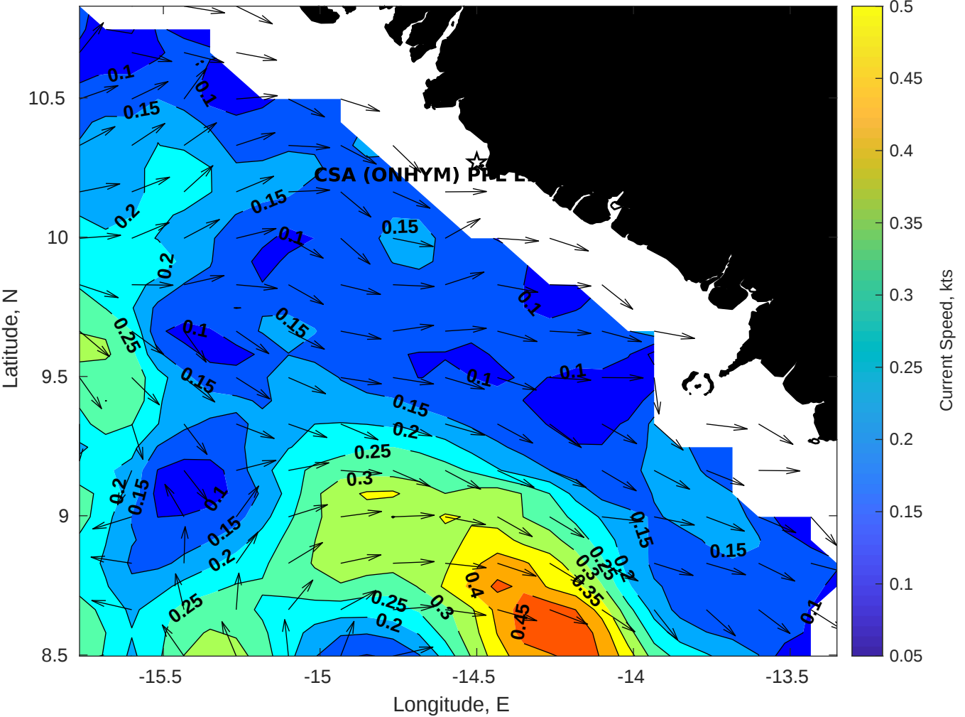
Surface Currents for CSA (ONHYM) PPL EBS - Guinea at 19-Jan-2026 00:00:00
