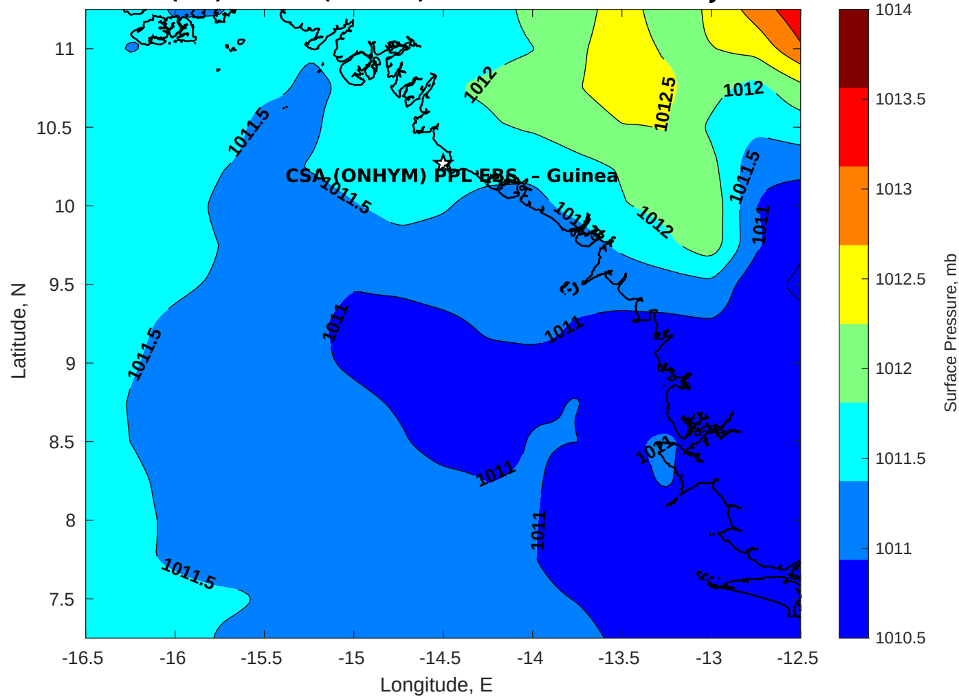
Surface Pressure (mb) for CSA (ONHYM) PPL EBS - Guinea at 22-Jan-2026 00:00:00
