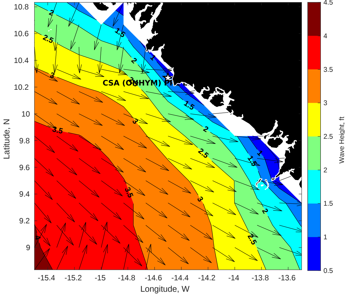
GFS Wave Height (ft) for CSA (ONHYM) PPL EBS - Guinea at 20-Jan-2026 09:00:00
