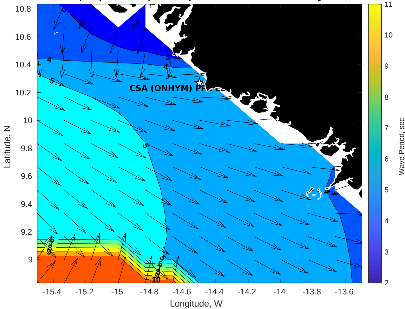
GFS Wave Period (sec) for CSA (ONHYM) PPL EBS - Guinea at 20-Jan-2026 09:00:00
