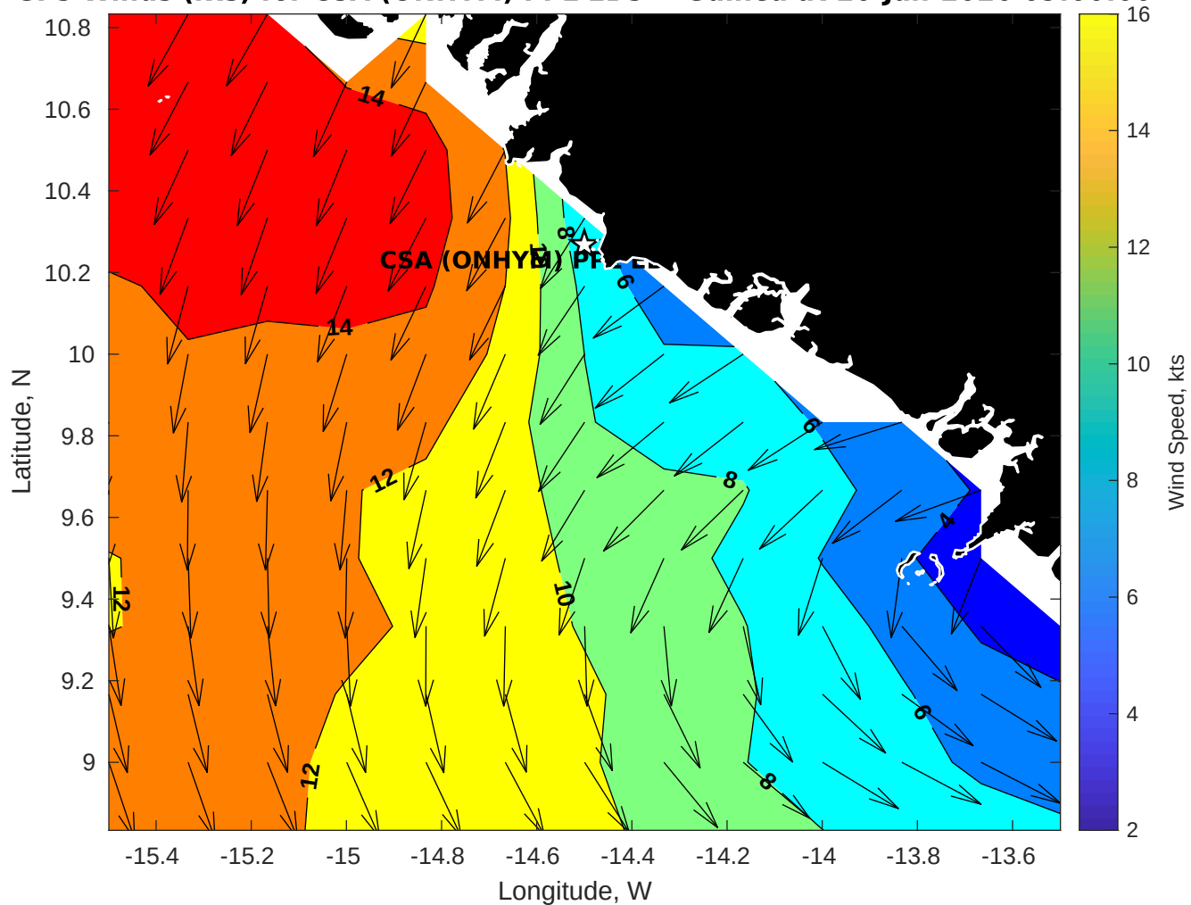
GFS Winds (kts) for CSA (ONHYM) PPL EBS - Guinea at 20-Jan-2026 09:00:00
