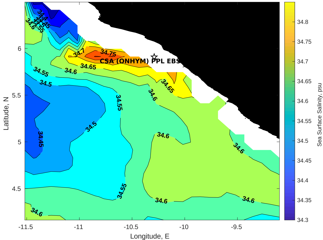
Surface Salinity for CSA (ONHYM) PPL EBS - Liberia at 19-Jan-2026 00:00:00
