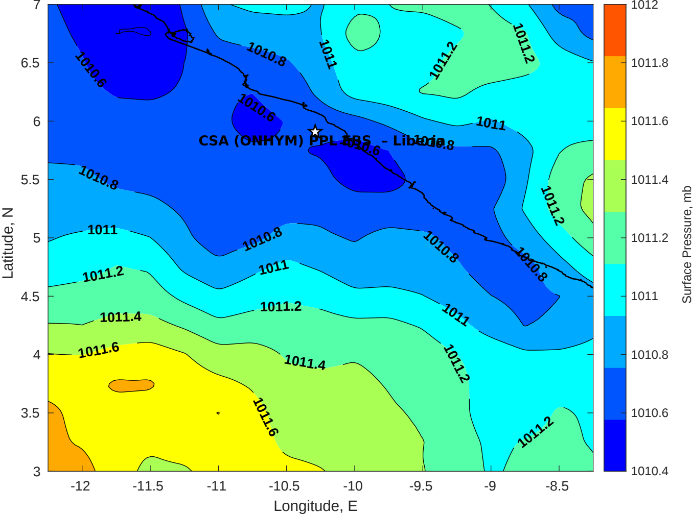
Surface Pressure (mb) for CSA (ONHYM) PPL EBS - Liberia at 20-Jan-2026 00:00:00
