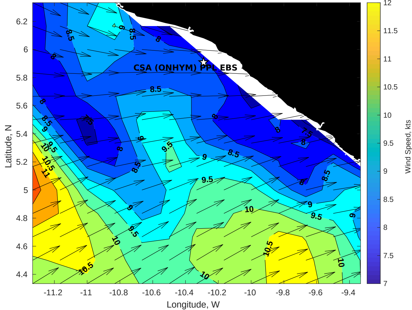
GFS Winds (kts) for CSA (ONHYM) PPL EBS - Liberia at 20-Jan-2026 09:00:00
