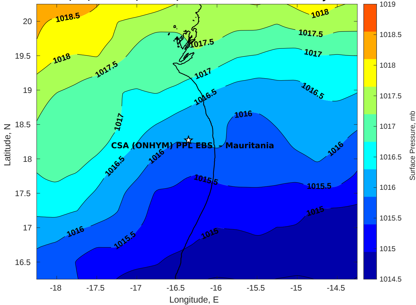
Surface Pressure (mb) for CSA (ONHYM) PPL EBS - Mauritania at 20-Jan-2026 00:00:00
