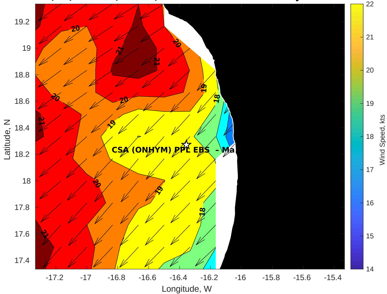
GFS Winds (kts) for CSA (ONHYM) PPL EBS - Mauritania at 20-Jan-2026 09:00:00
