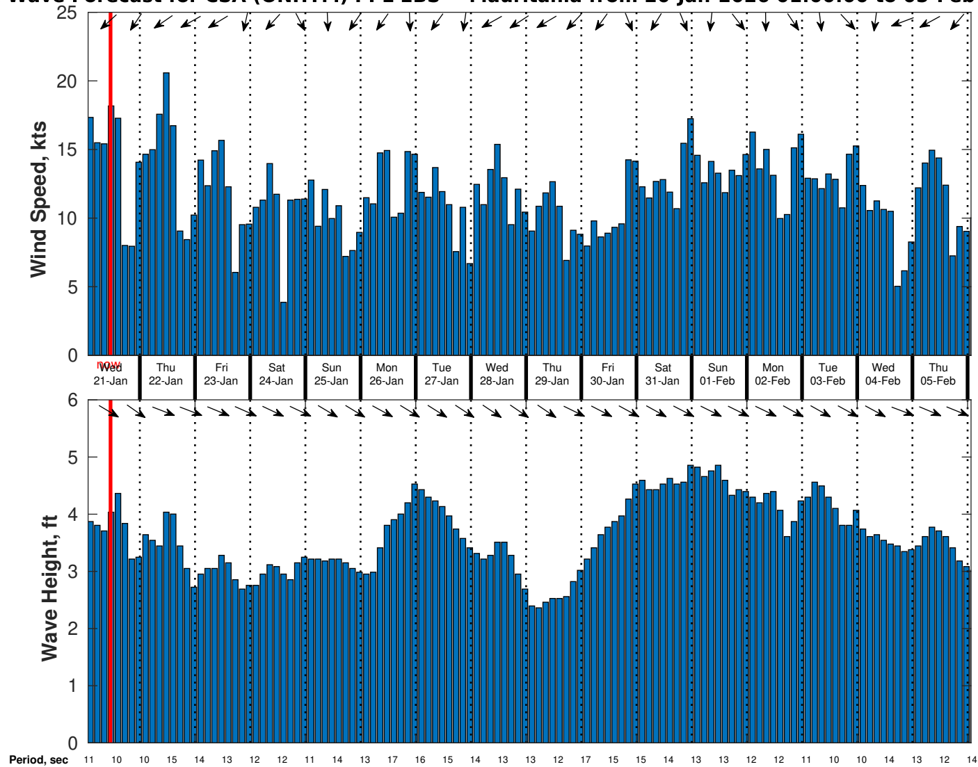
Wind & Wave Forecast for CSA (ONHYM) PPL EBS - Mauritania from 20-Jan-2026 01:00:00 to 05-Feb-2026 01:00:00
