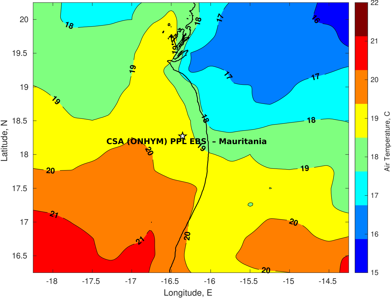
Air Temperature (C) for CSA (ONHYM) PPL EBS - Mauritania at 20-Jan-2026
