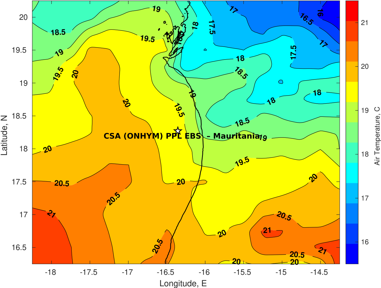
Air Temperature (C) for CSA (ONHYM) PPL EBS - Mauritania at 20-Jan-2026
