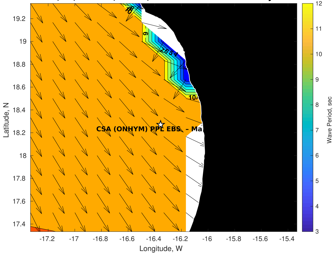
GFS Wave Period (sec) for CSA (ONHYM) PPL EBS - Mauritania at 20-Jan-2026 09:00:00
