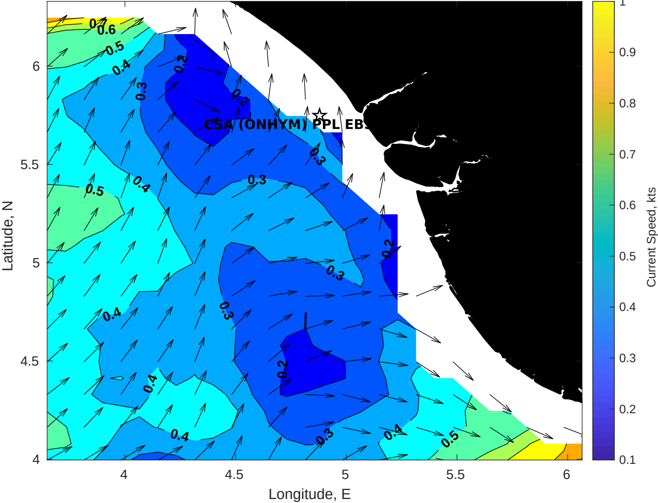
Surface Currents for CSA (ONHYM) PPL EBS - Nigeria at 19-Jan-2026 00:00:00
