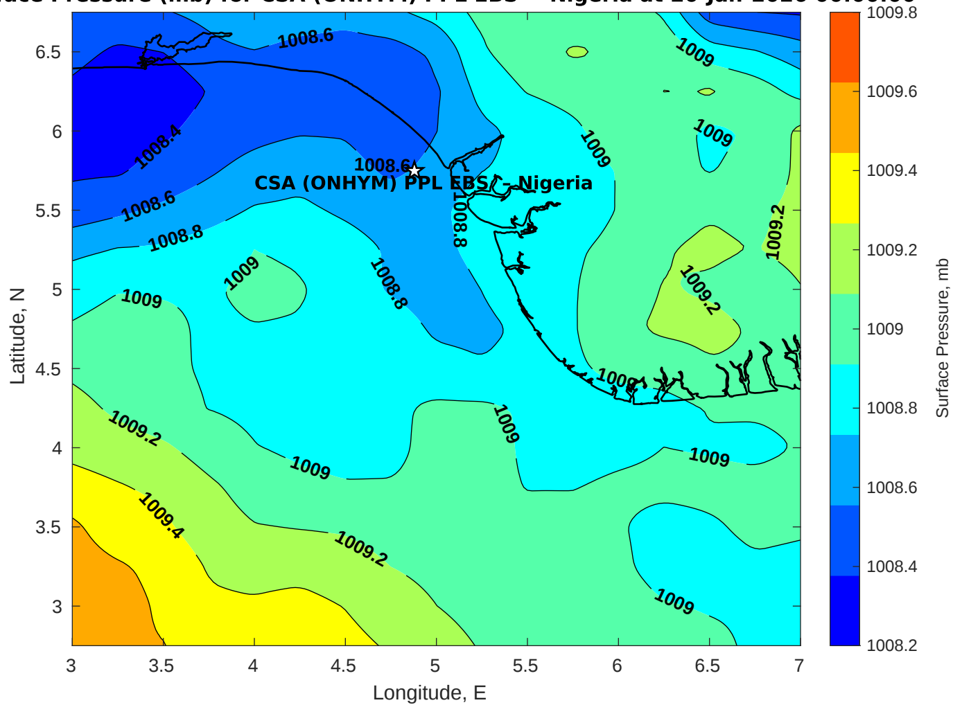
Surface Pressure (mb) for CSA (ONHYM) PPL EBS - Nigeria at 20-Jan-2026 00:00:00
