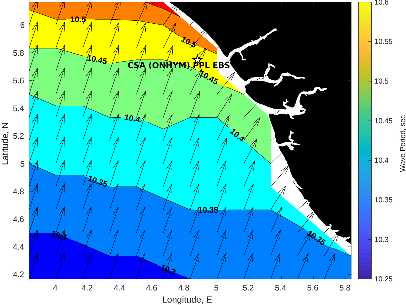
GFS Wave Period (sec) for CSA (ONHYM) PPL EBS - Nigeria at 20-Jan-2026 09:00:00
