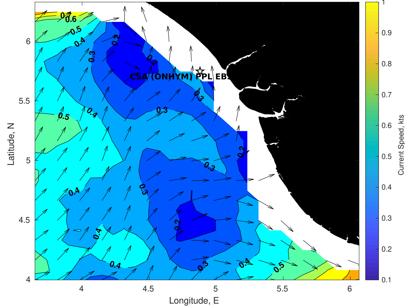
Surface Currents for CSA (ONHYM) PPL EBS - Nigeria at 19-Jan-2026 00:00:00
