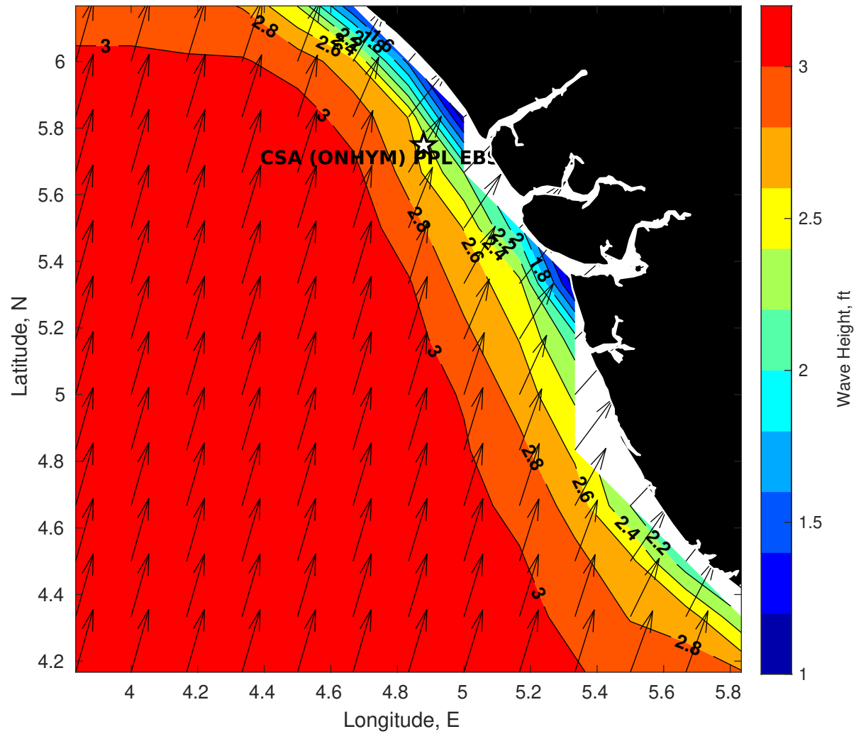
GFS Wave Height (ft) for CSA (ONHYM) PPL EBS - Nigeria at 20-Jan-2026 09:00:00
