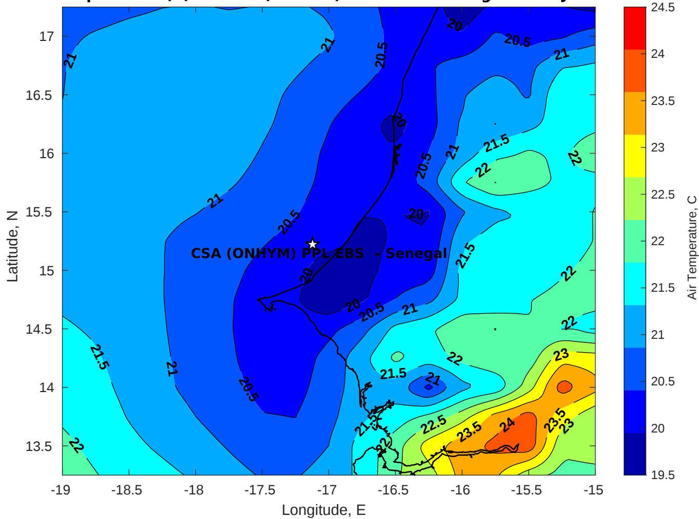
Air Temperature (C) for CSA (ONHYM) PPL EBS - Senegal at 20-Jan-2026
