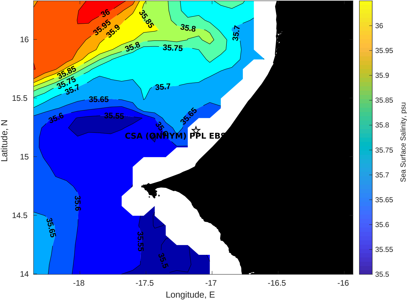
Surface Salinity for CSA (ONHYM) PPL EBS - Senegal at 19-Jan-2026 00:00:00
