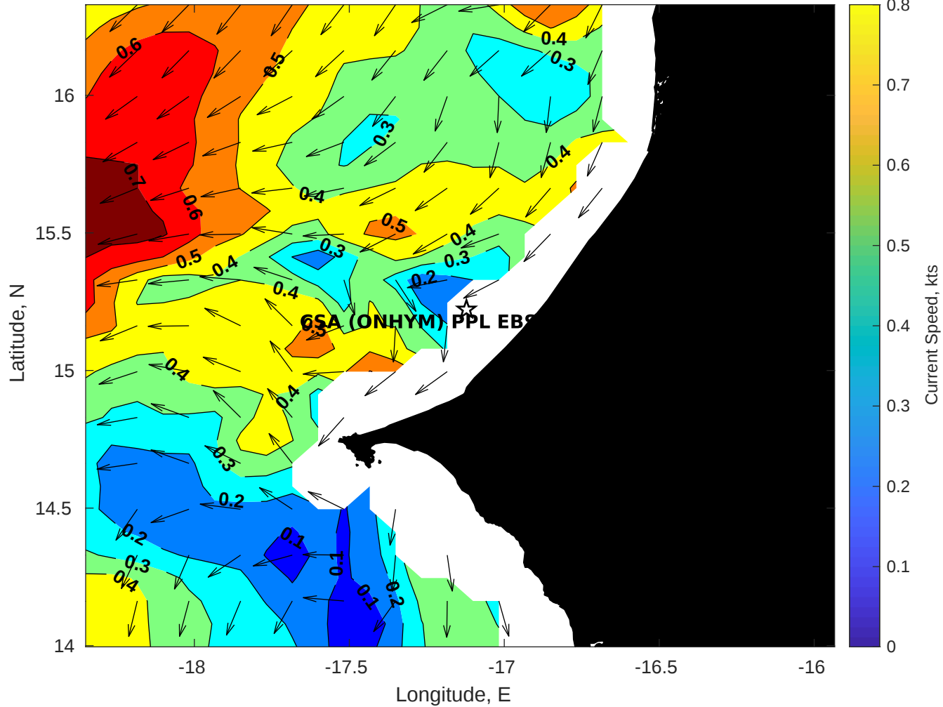
Surface Currents for CSA (ONHYM) PPL EBS - Senegal at 19-Jan-2026 00:00:00
