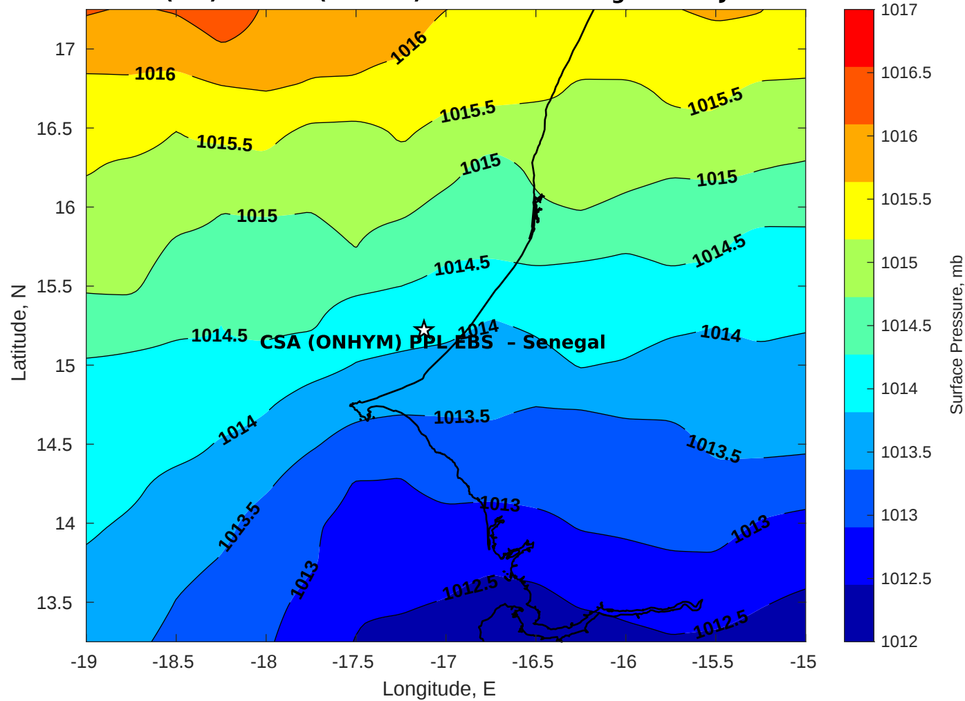
Surface Pressure (mb) for CSA (ONHYM) PPL EBS - Senegal at 22-Jan-2026 00:00:00
