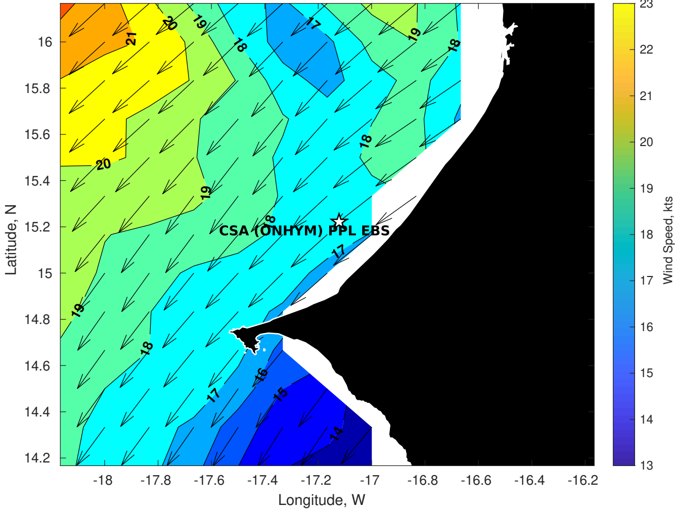
GFS Winds (kts) for CSA (ONHYM) PPL EBS - Senegal at 20-Jan-2026 09:00:00
