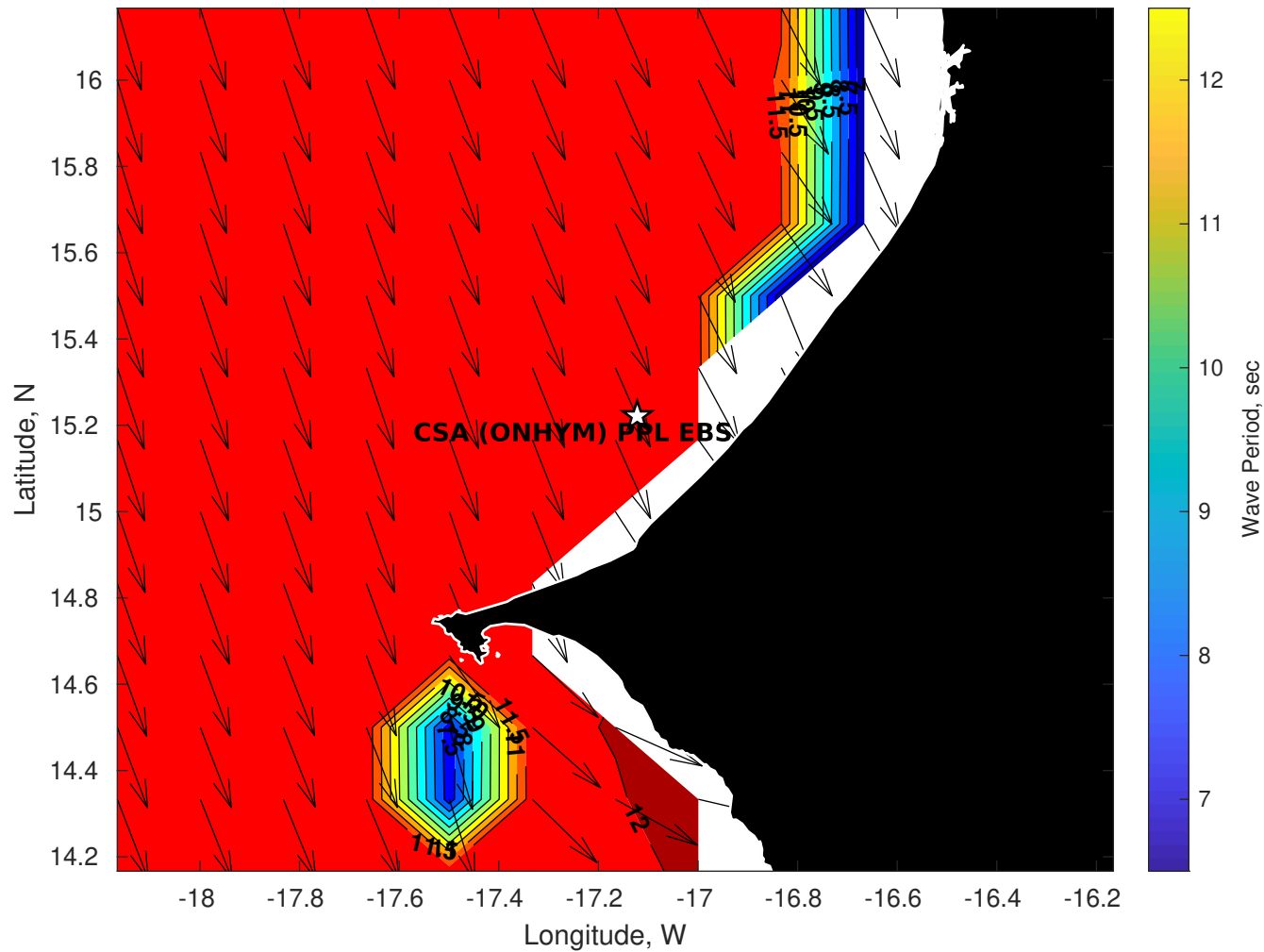
GFS Wave Period (sec) for CSA (ONHYM) PPL EBS - Senegal at 20-Jan-2026 09:00:00
