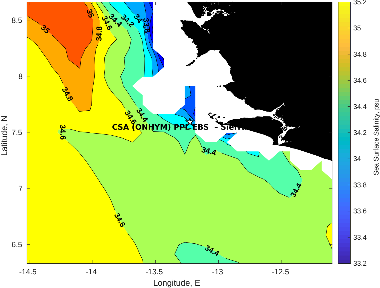
Surface Salinity for CSA (ONHYM) PPL EBS - Sierra Leone at 19-Jan-2026 00:00:00
