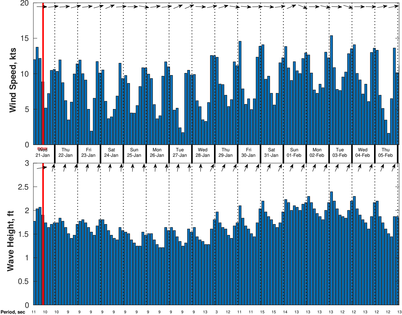
Wind & Wave Forecast for CSA (ONHYM) PPL EBS - Sierra Leone from 20-Jan-2026 01:00:00 to 05-Feb-2026 01:00:00
