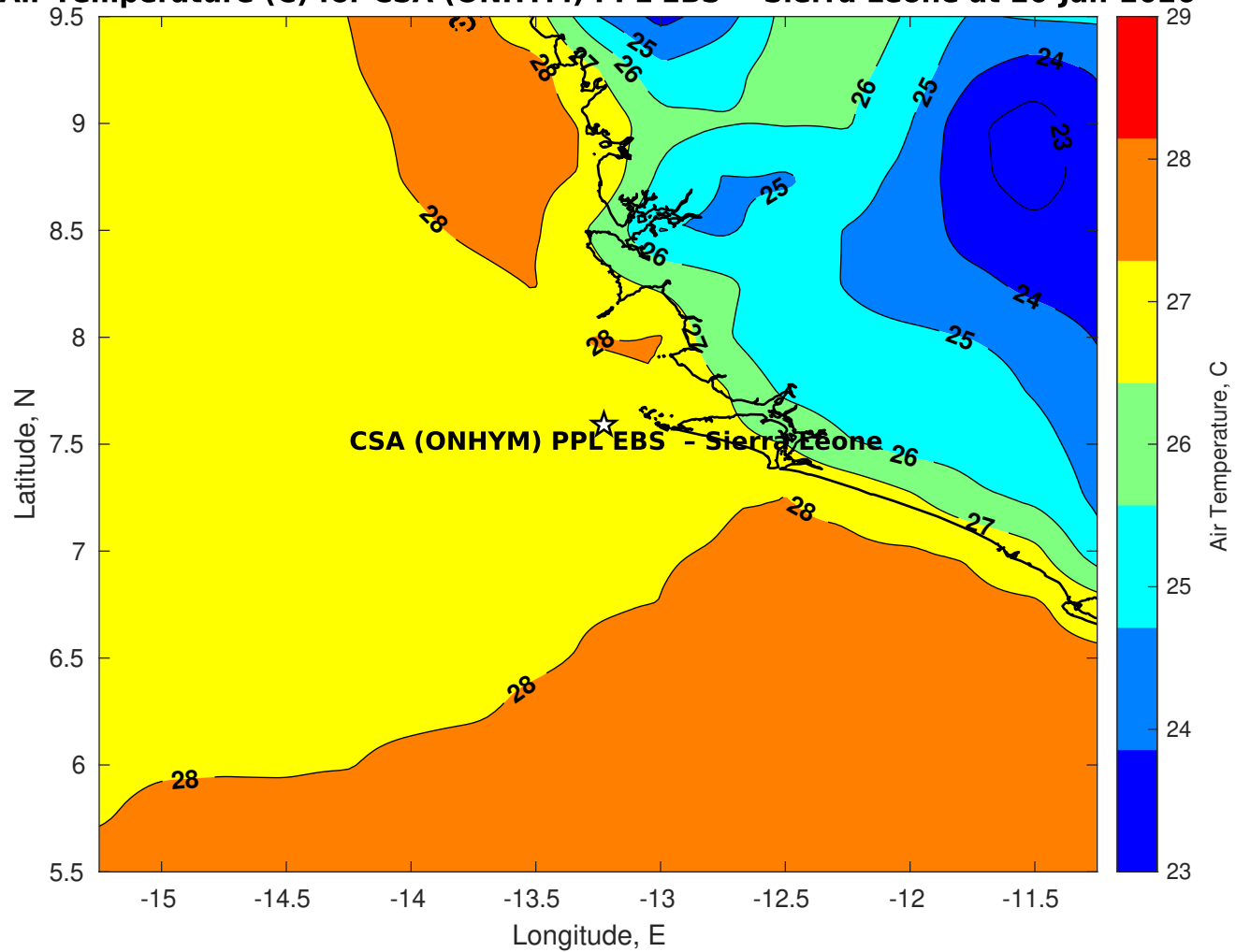
Air Temperature (C) for CSA (ONHYM) PPL EBS - Sierra Leone at 20-Jan-2026
