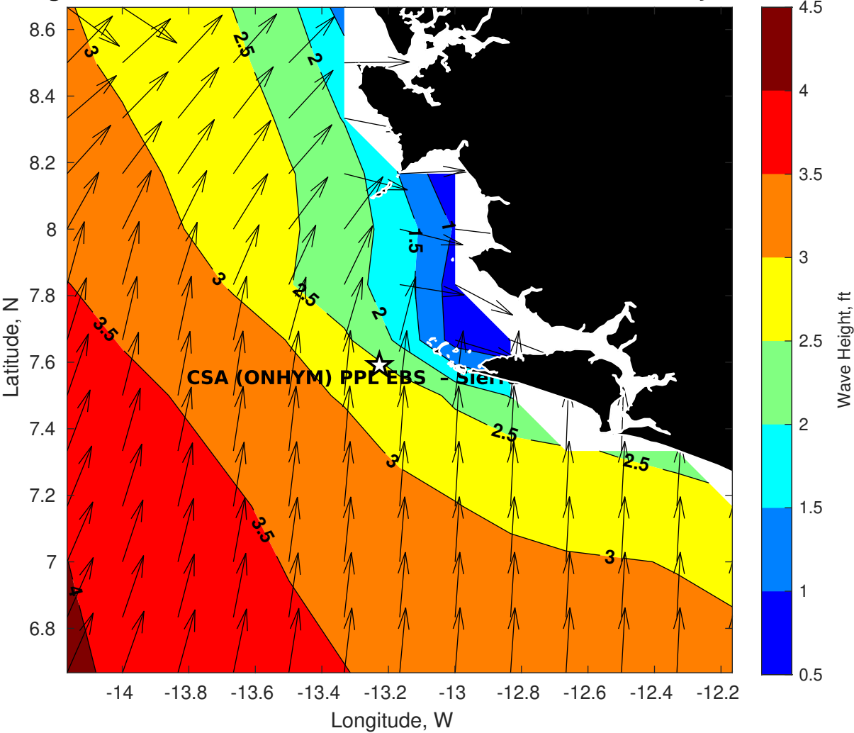
GFS Wave Height (ft) for CSA (ONHYM) PPL EBS - Sierra Leone at 20-Jan-2026 09:00:00
