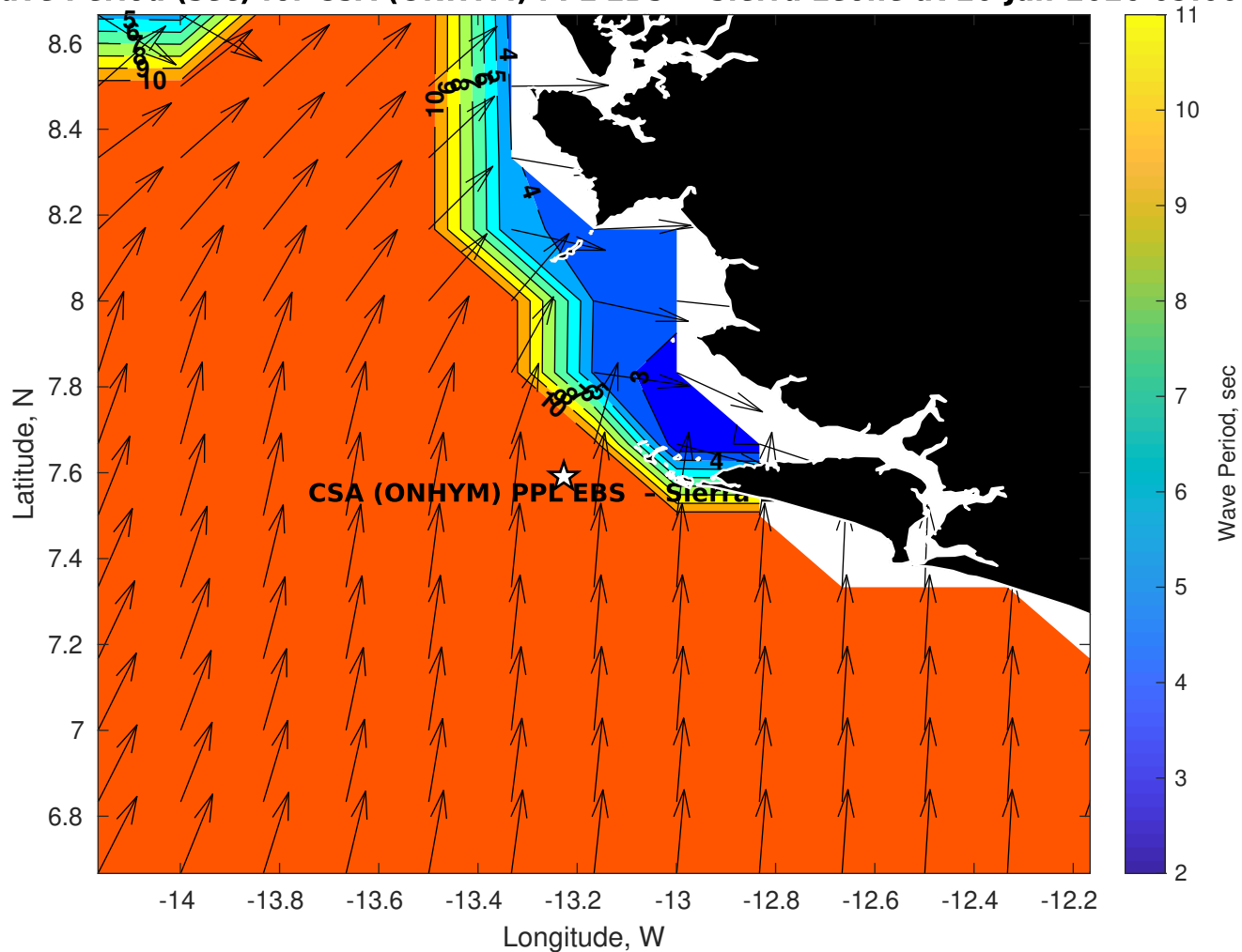
GFS Wave Period (sec) for CSA (ONHYM) PPL EBS - Sierra Leone at 20-Jan-2026 09:00:00
