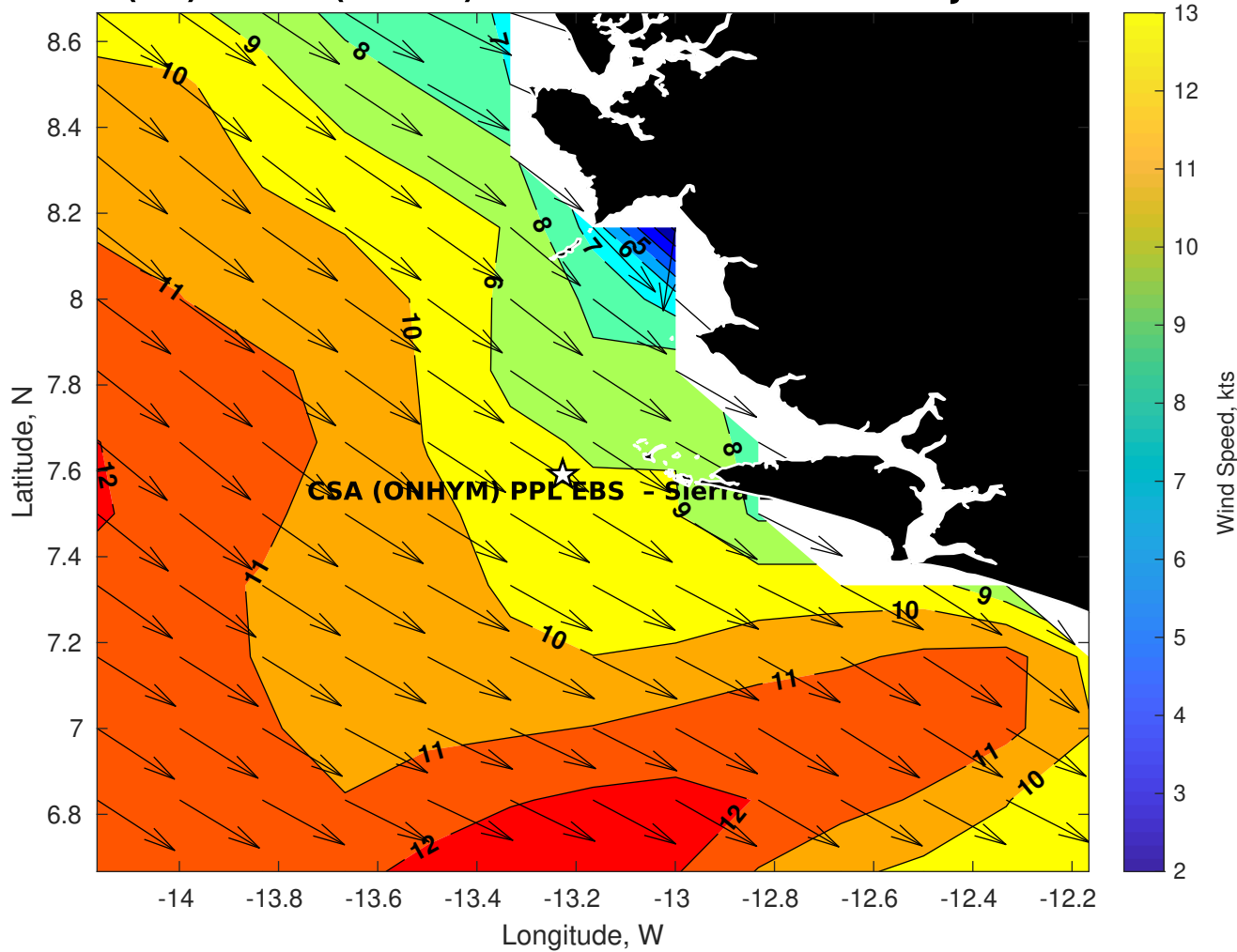
GFS Winds (kts) for CSA (ONHYM) PPL EBS - Sierra Leone at 20-Jan-2026 09:00:00
