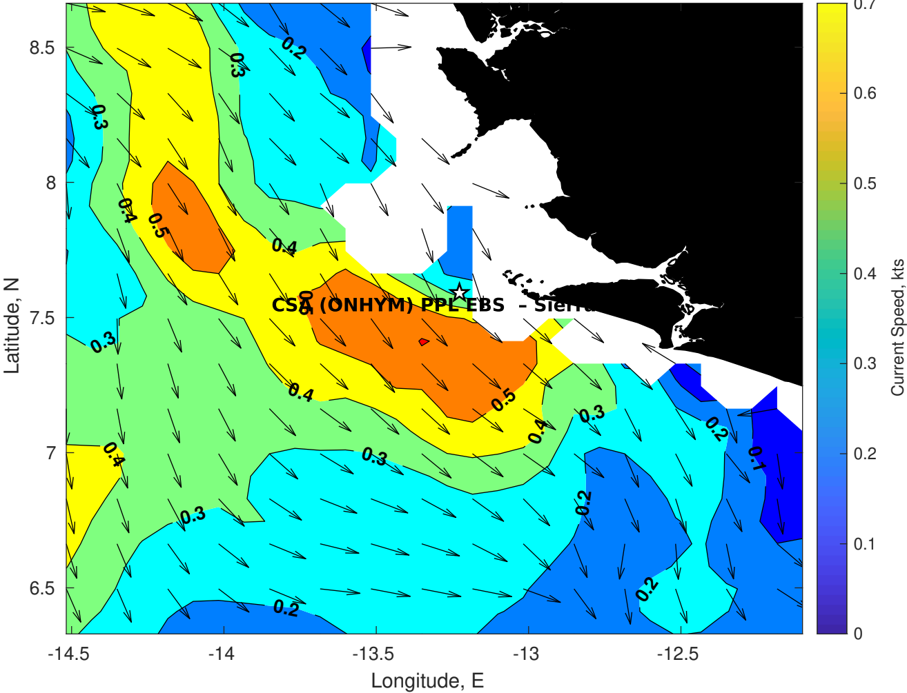
Surface Currents for CSA (ONHYM) PPL EBS - Sierra Leone at 19-Jan-2026 00:00:00
