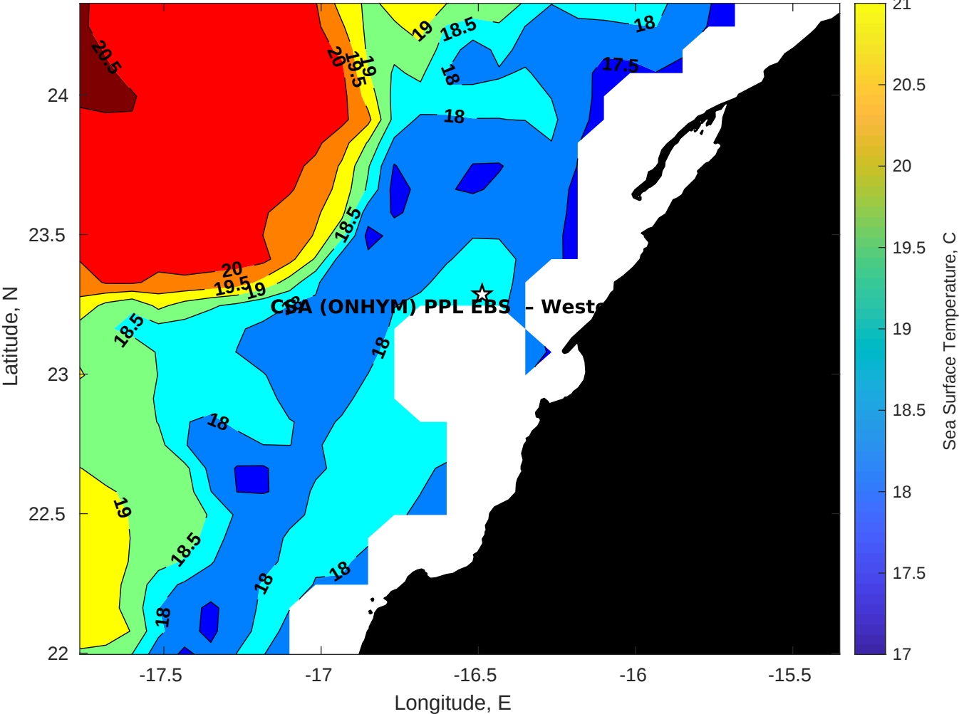
SST for CSA (ONHYM) PPL EBS - Western Sahara at 19-Jan-2026 00:00:00
