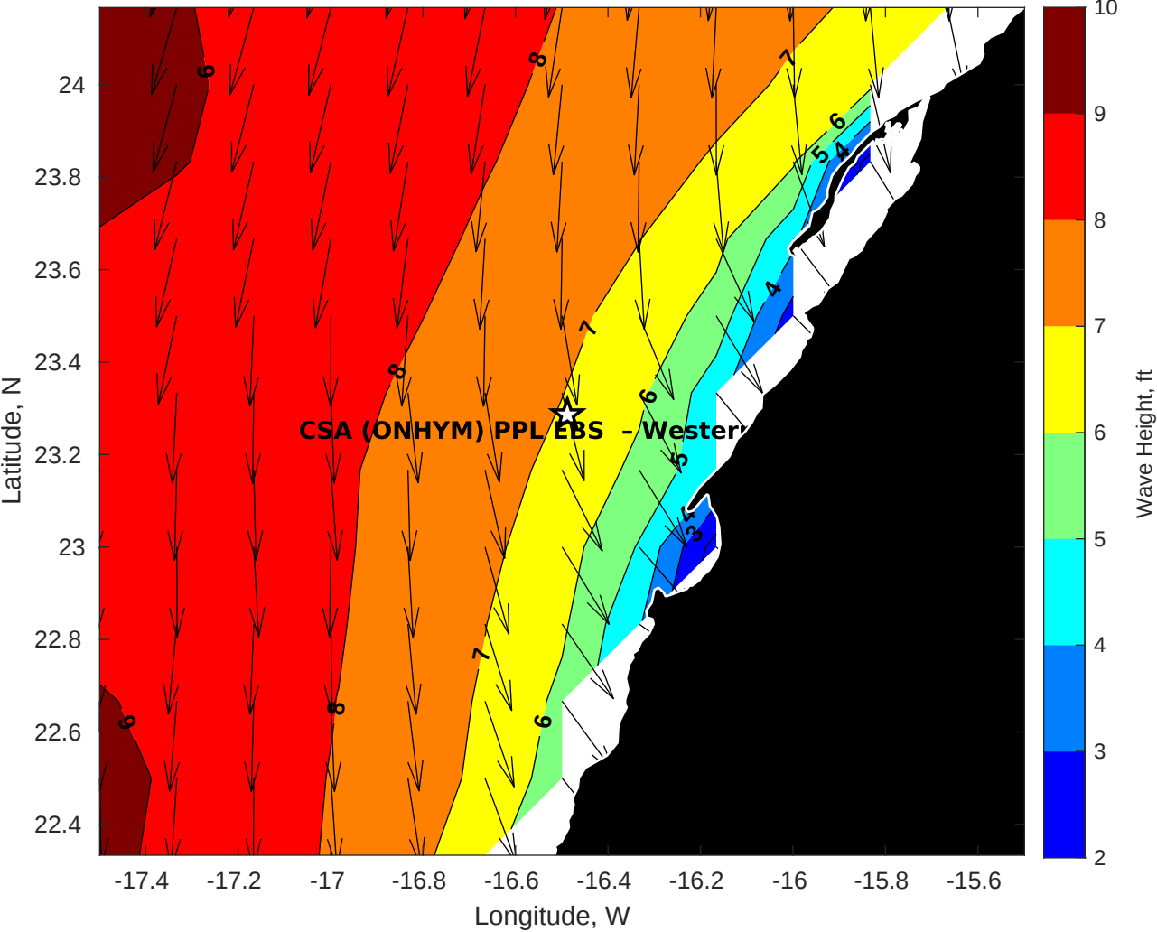
GFS Wave Height (ft) for CSA (ONHYM) PPL EBS - Western Sahara at 20-Jan-2026 09:00:00
