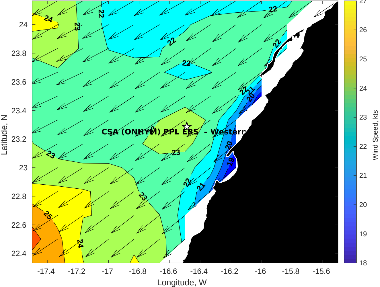
GFS Winds (kts) for CSA (ONHYM) PPL EBS - Western Sahara at 20-Jan-2026 09:00:00
