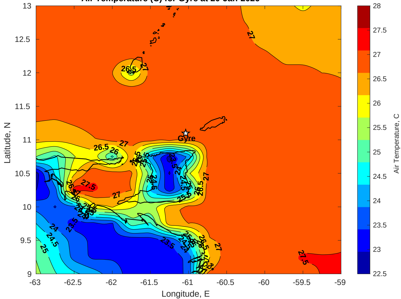
Air Temperature (C) for Gyre at 20-Jan-2026
