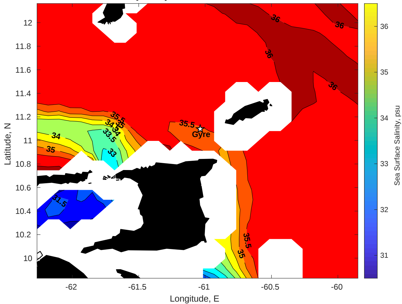
Surface Salinity for Gyre at 19-Jan-2026 00:00:00
