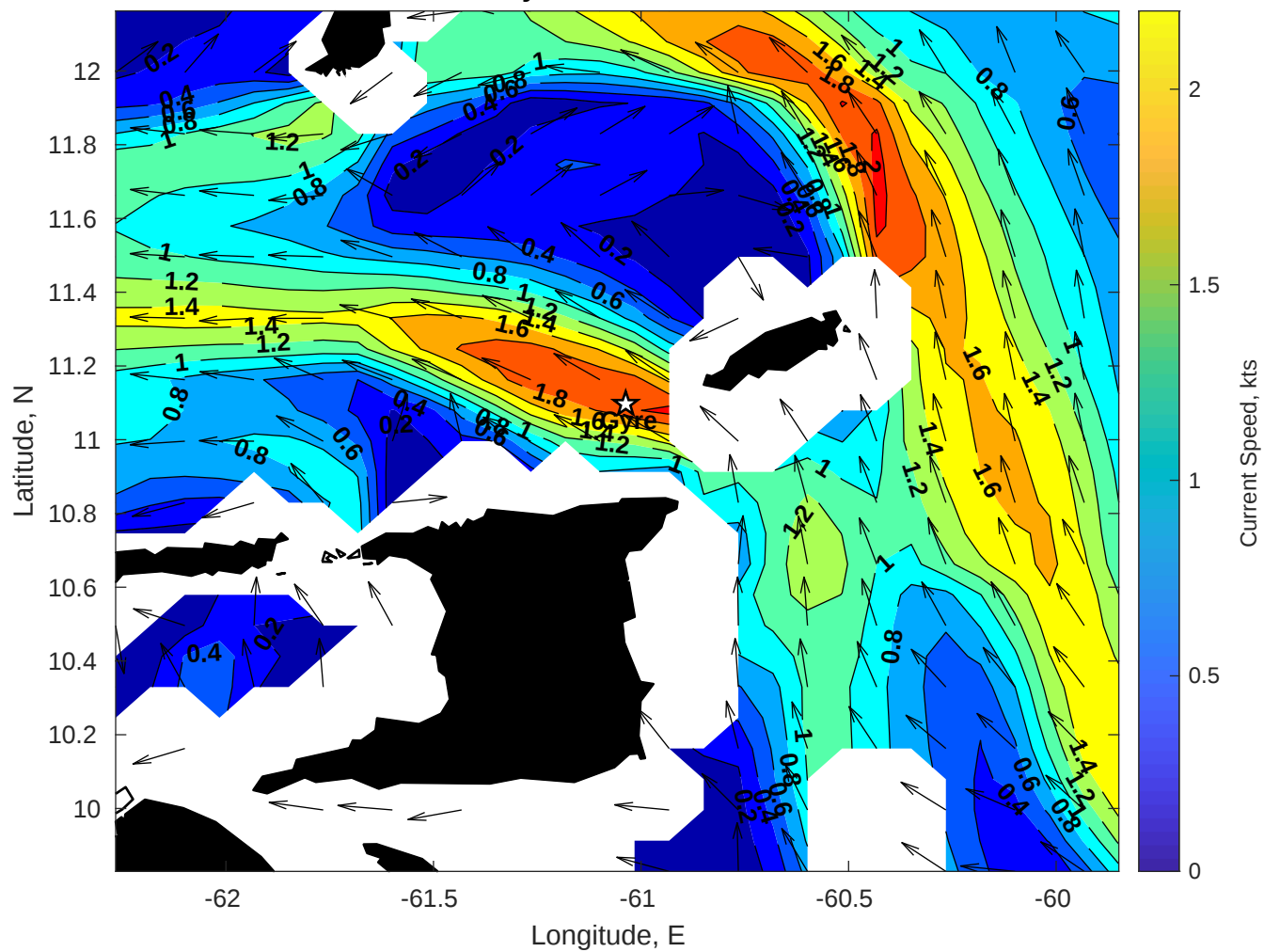
Surface Currents for Gyre at 19-Jan-2026 00:00:00
