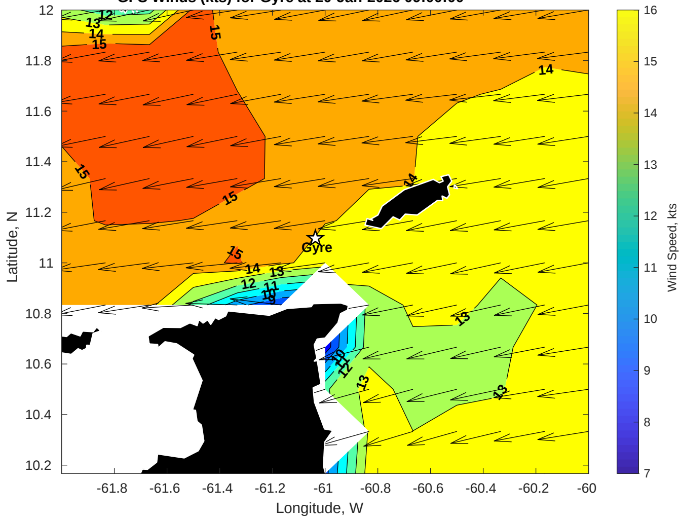
GFS Winds (kts) for Gyre at 20-Jan-2026 09:00:00
