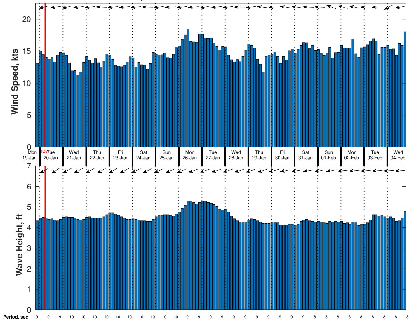
Wind & Wave Forecast for Gyre from 19-Jan-2026 20:00:00 to 04-Feb-2026 20:00:00
