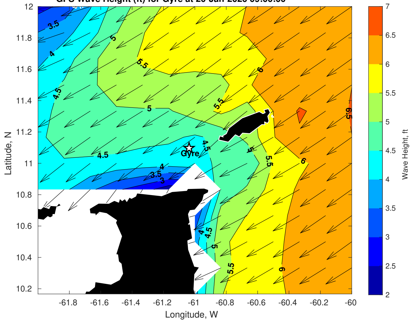
GFS Wave Height (ft) for Gyre at 20-Jan-2026 09:00:00
