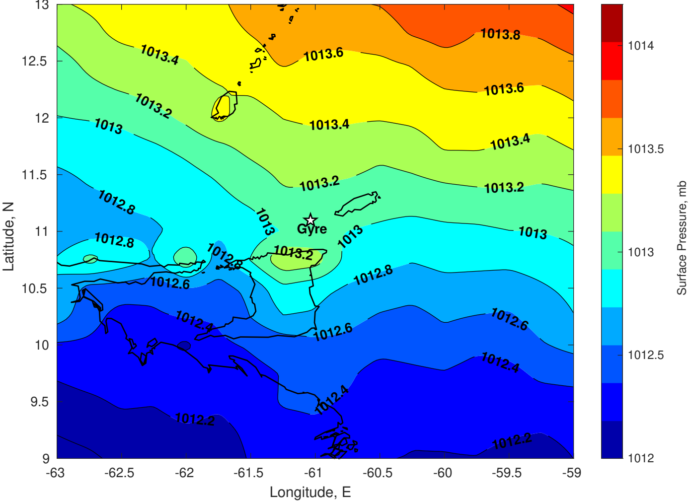
Surface Pressure (mb) for Gyre at 20-Jan-2026 00:00:00
