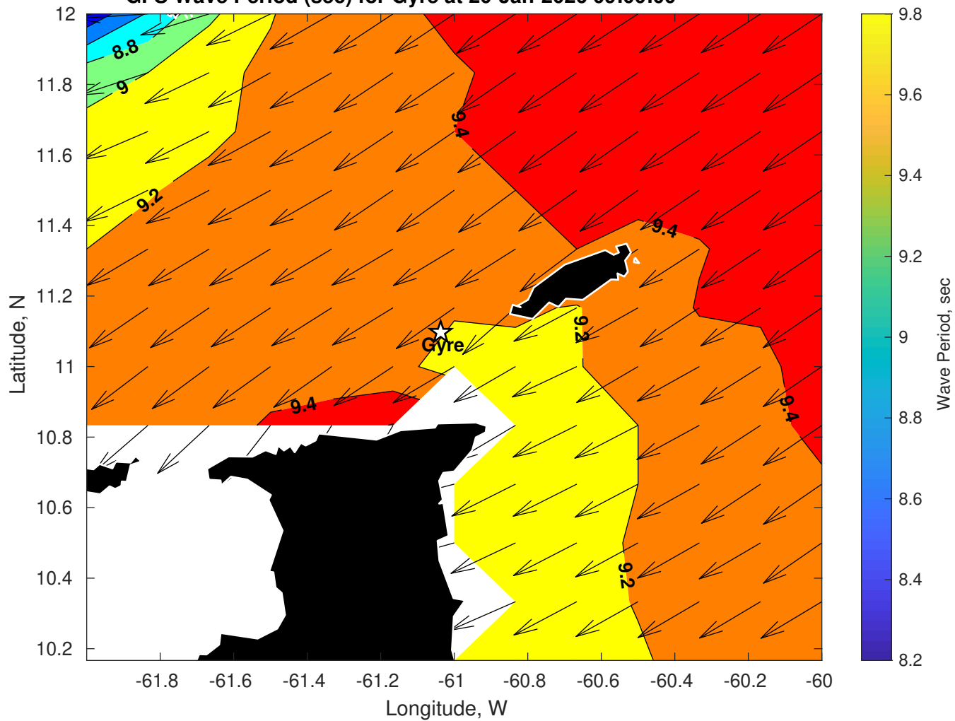
GFS Wave Period (sec) for Gyre at 20-Jan-2026 09:00:00
