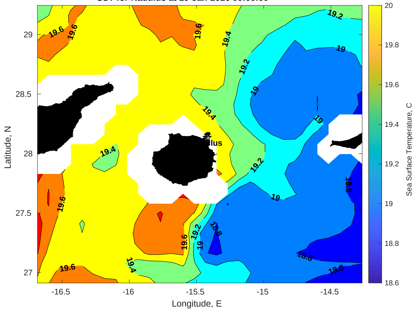
SST for Nautilus at 19-Jan-2026 00:00:00
