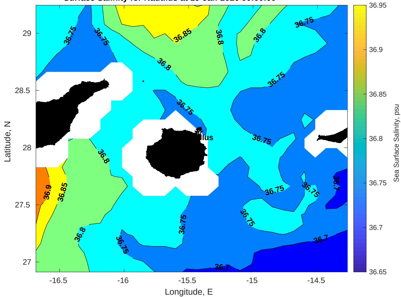
Surface Salinity for Nautilus at 19-Jan-2026 00:00:00
