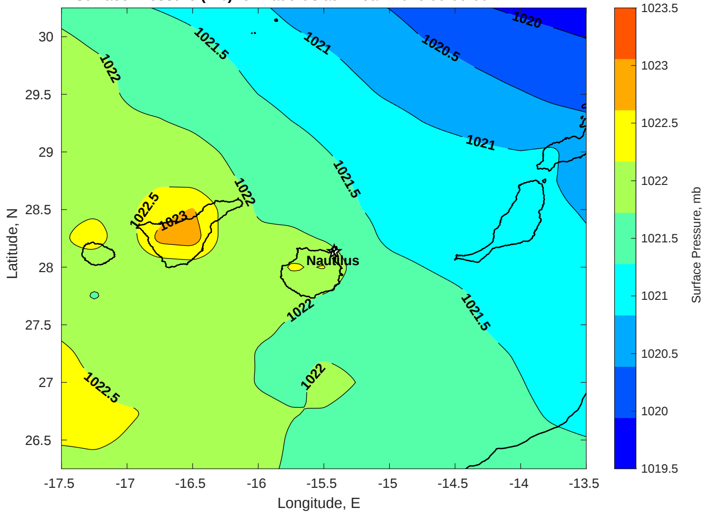
Surface Pressure (mb) for Nautilus at 22-Jan-2026 00:00:00
